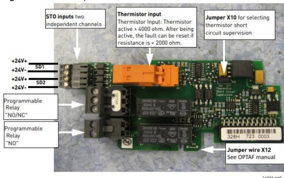
Figure 1. The OPTAF option board
