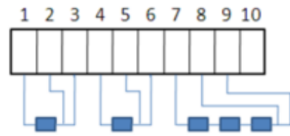
Three-wire configuration
