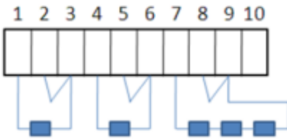
Two-wire configuration
