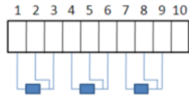
Three-wire configuration
