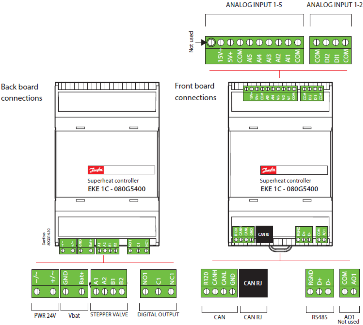
EKE 1C – Front board connection overview
