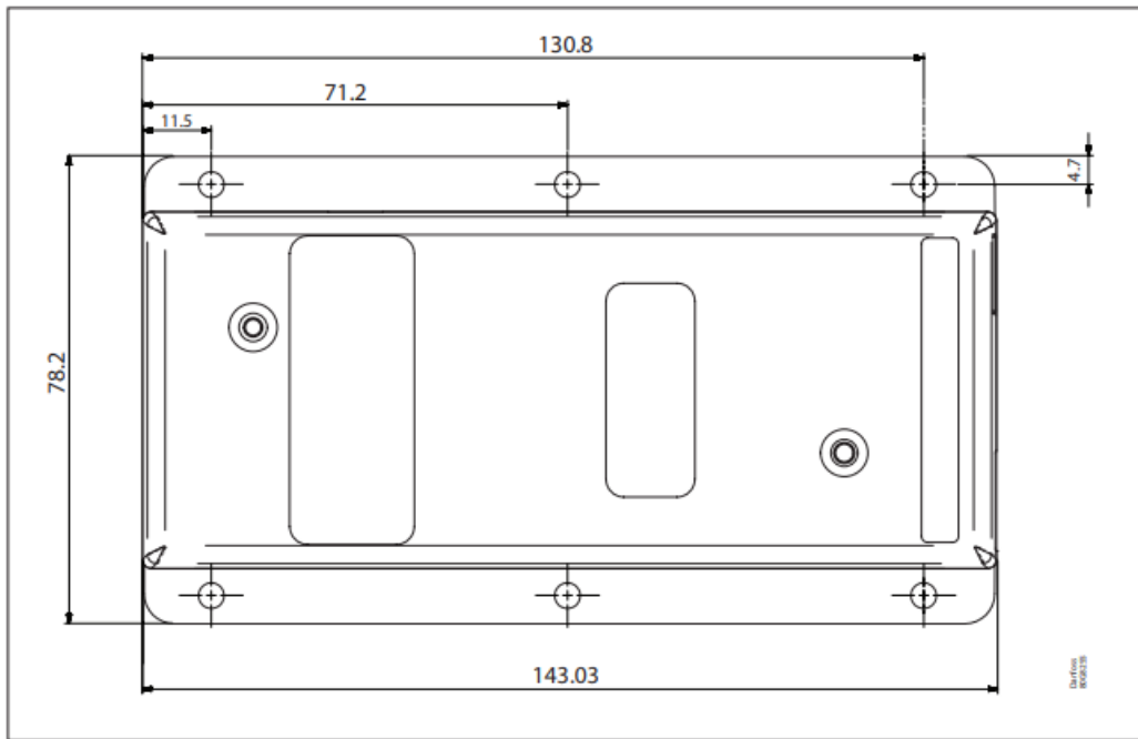
Fig. 10: Top view
