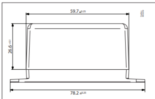
Fig. 11: Rear view
