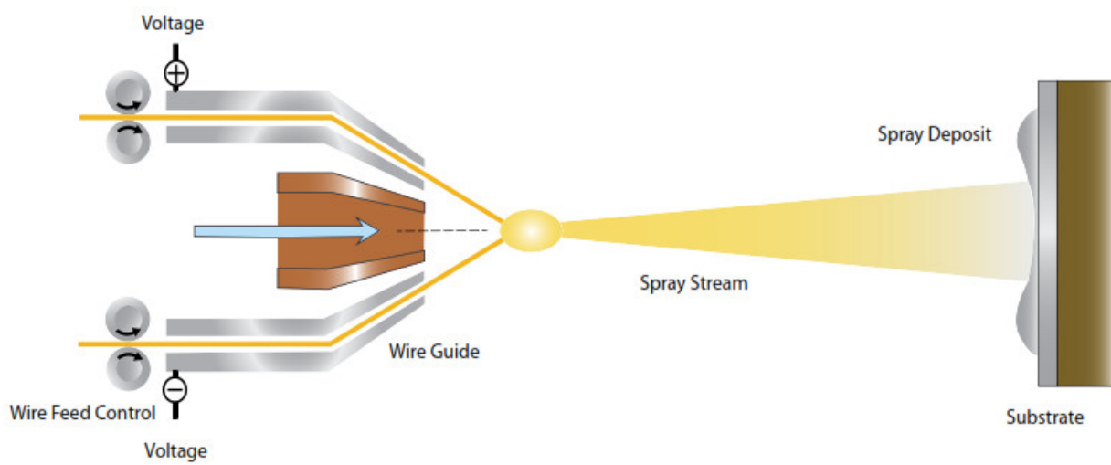
Figure 1 - Illustration of ZAS applied onto MPE tube surface
