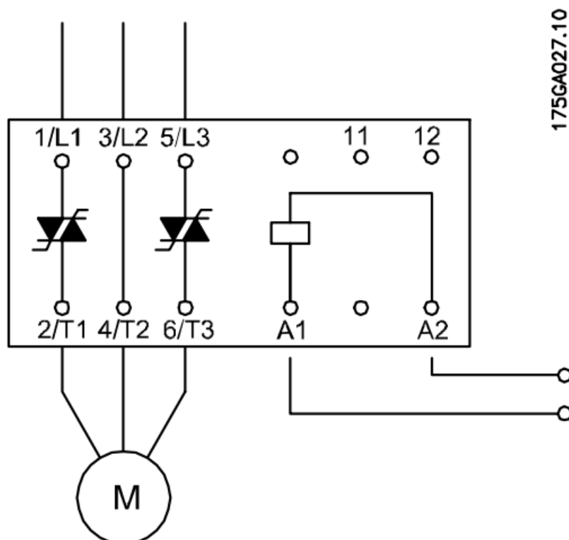
Illustration 1.2 MCD 100 – 007 / MCD 100 – 011
