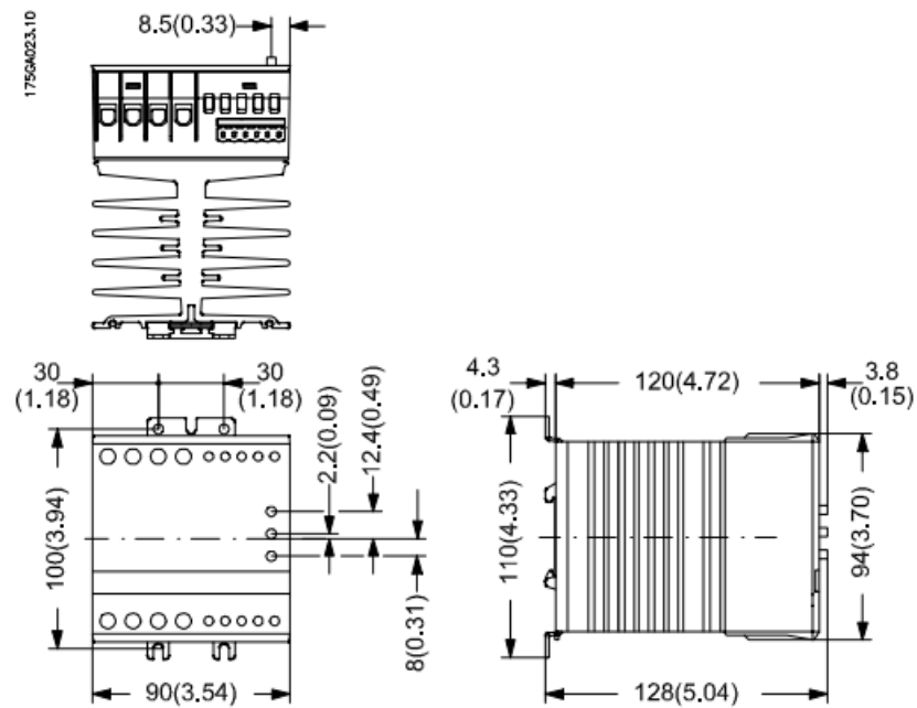
Illustration 1.5 MCD 100 - 011
