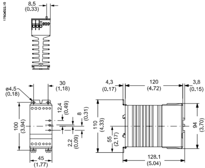
Illustration 1.4 MCD 100 - 007
