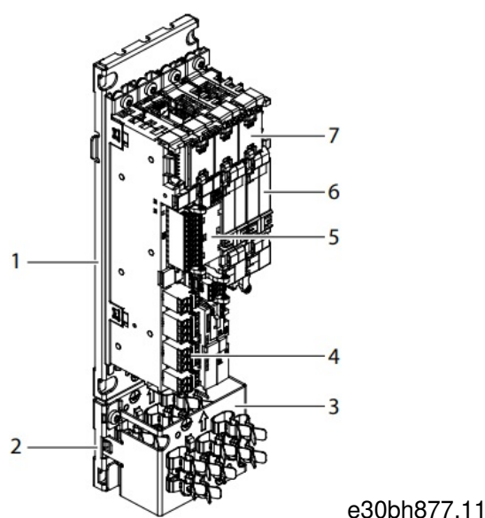
Figure 5: Example of the Modular Control Unit
