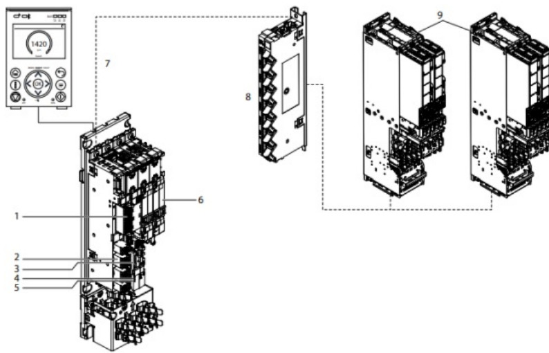
Figure 1: Interfaces of iC7 System Module
