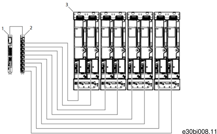
Figure 4: Example Control Connection with a Star Coupler Board: 8 Power Units in Parallel
