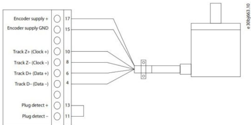
Illustration 12: Wiring Configuration for 2-Track BiSS Encoder
