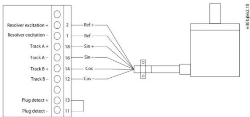
Illustration 7: Wiring Configuration for Resolver
