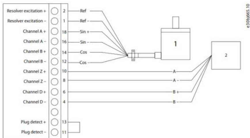
Illustration 8: Wiring Configuration for Resolver with Mirror Out
