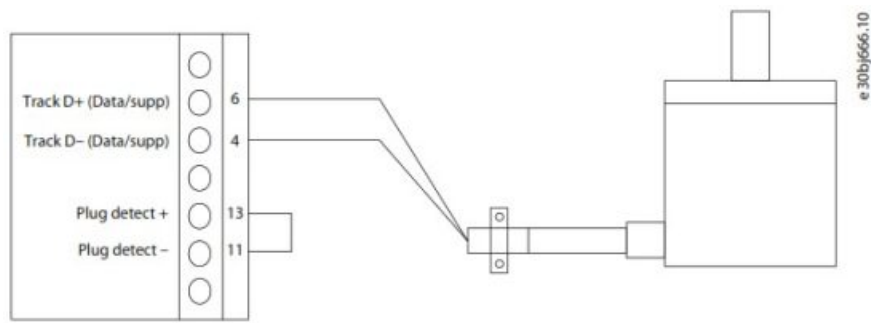
Illustration 13: Wiring Configuration for HIPERFACE DSL Encoder
