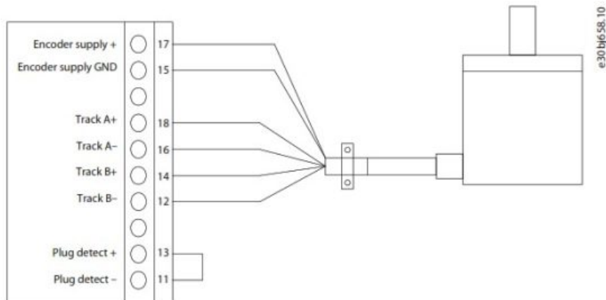
Illustration 9: Wiring Configuration for SinCos Encoder
