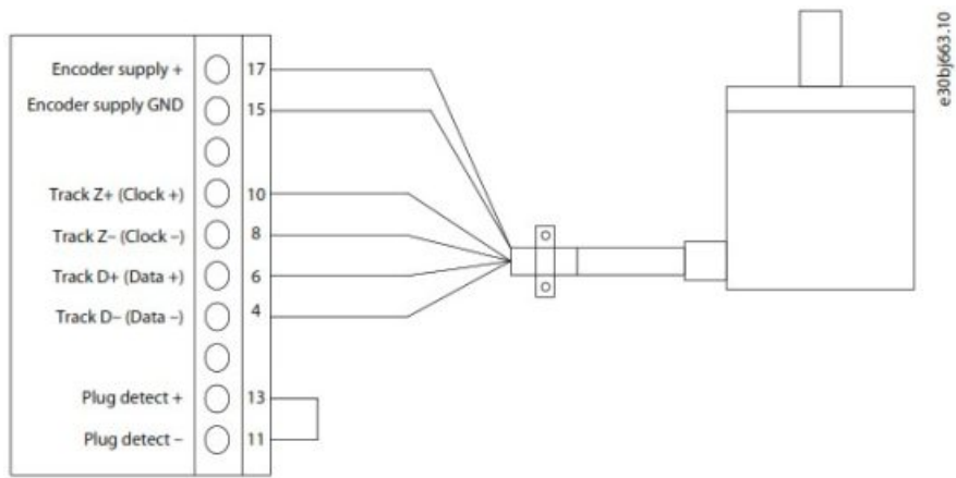
Illustration 10: Wiring Configuration for 2-Track SSI Encoder
