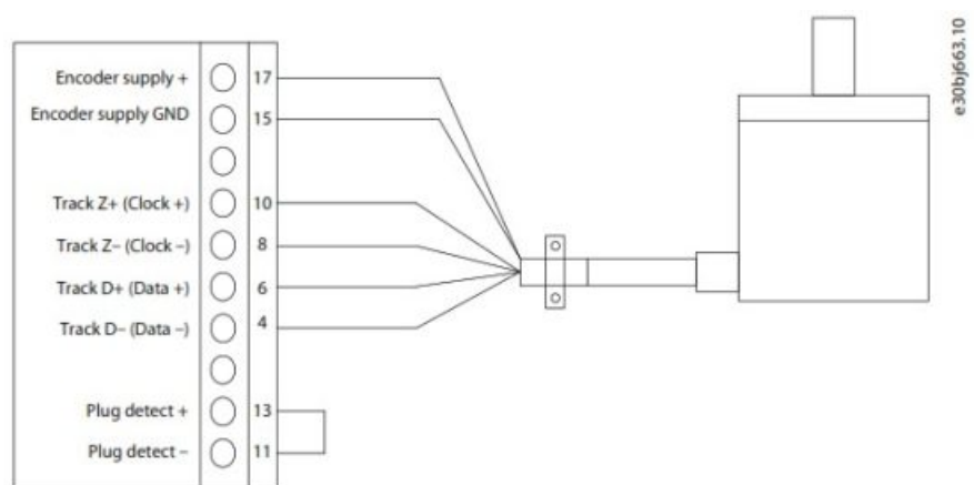
Illustration 11: Wiring Configuration for 2-Track EnDat Encoder
