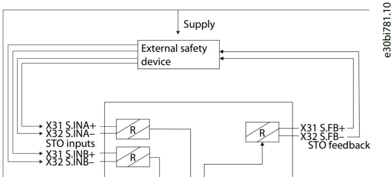
Illustration 3: STO Feedback Example (1/2)
