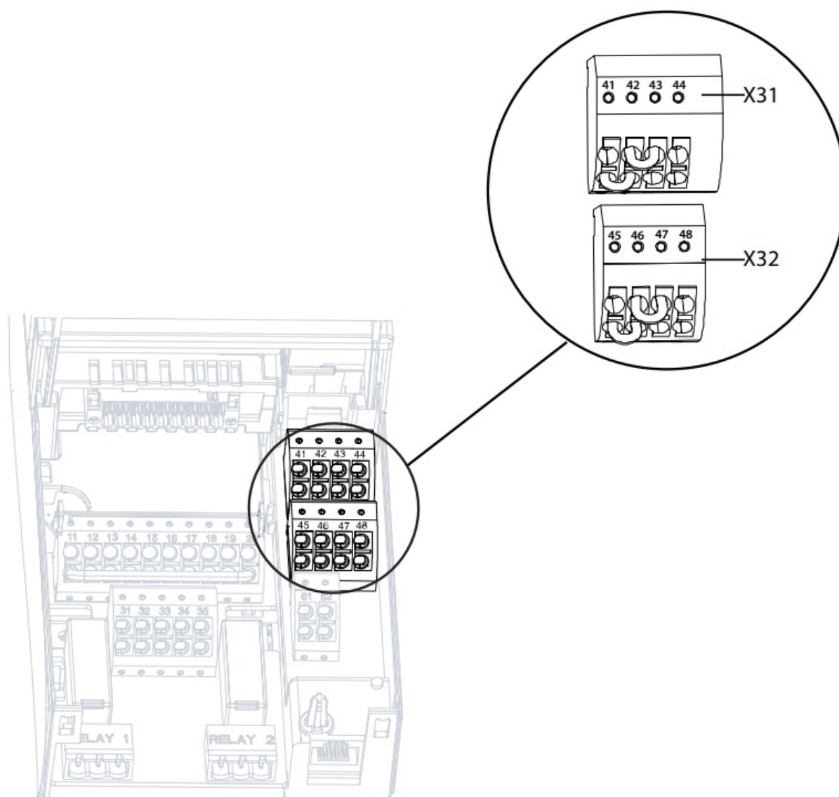
Illustration 5: Functional Safety Terminals
