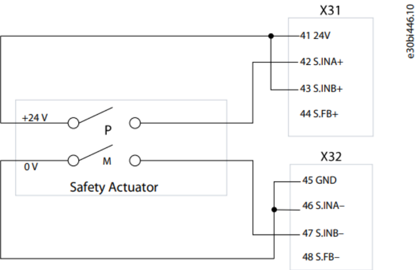
Illustration 8: STO Connection Example for Using Different Polarities
