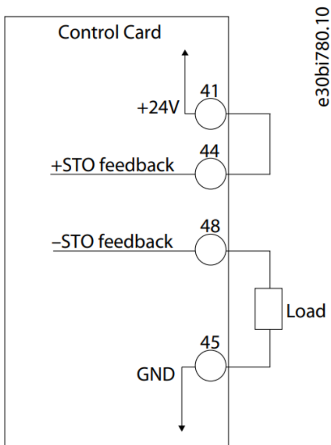
Illustration 4: STO Feedback Example (2/2)
