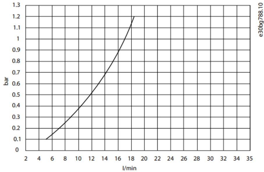
Illustration 8: Pressure Drop with Water, LC12L
