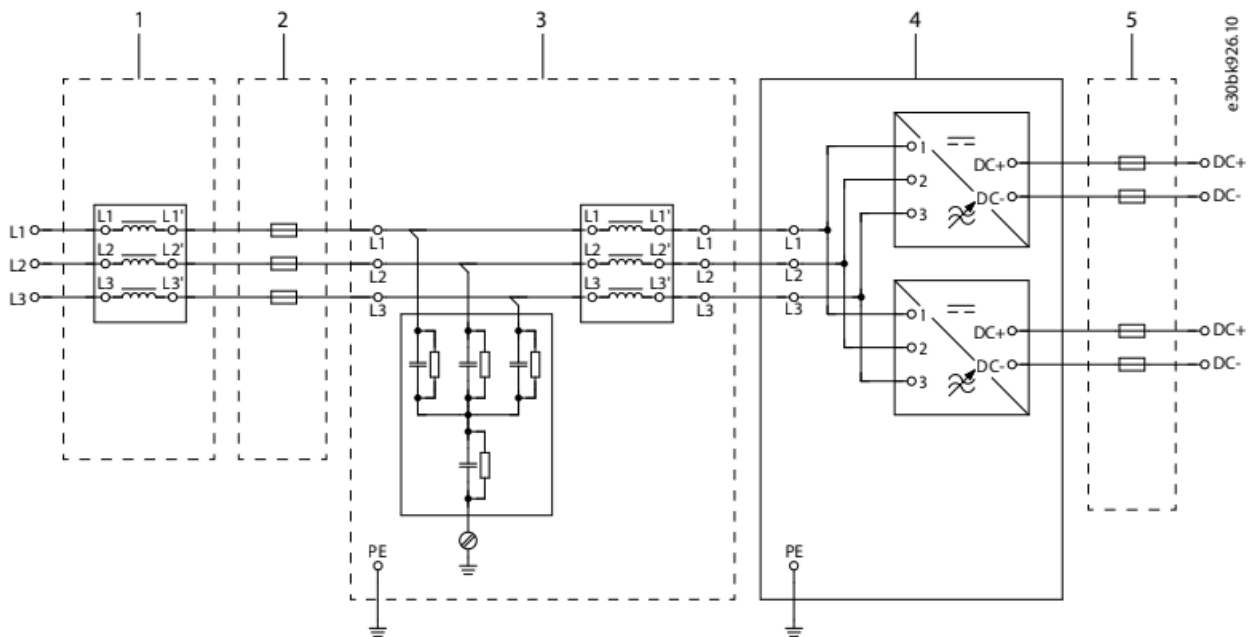
Illustration 17: Wiring Diagram, LC12L
