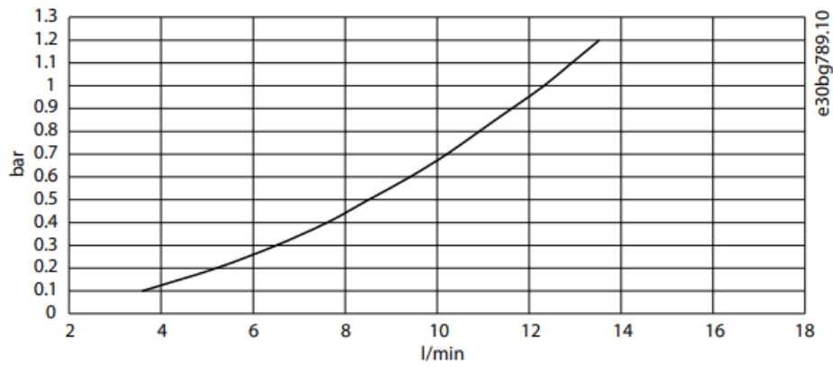
Illustration 7: Pressure Drop with Water, LC10L
