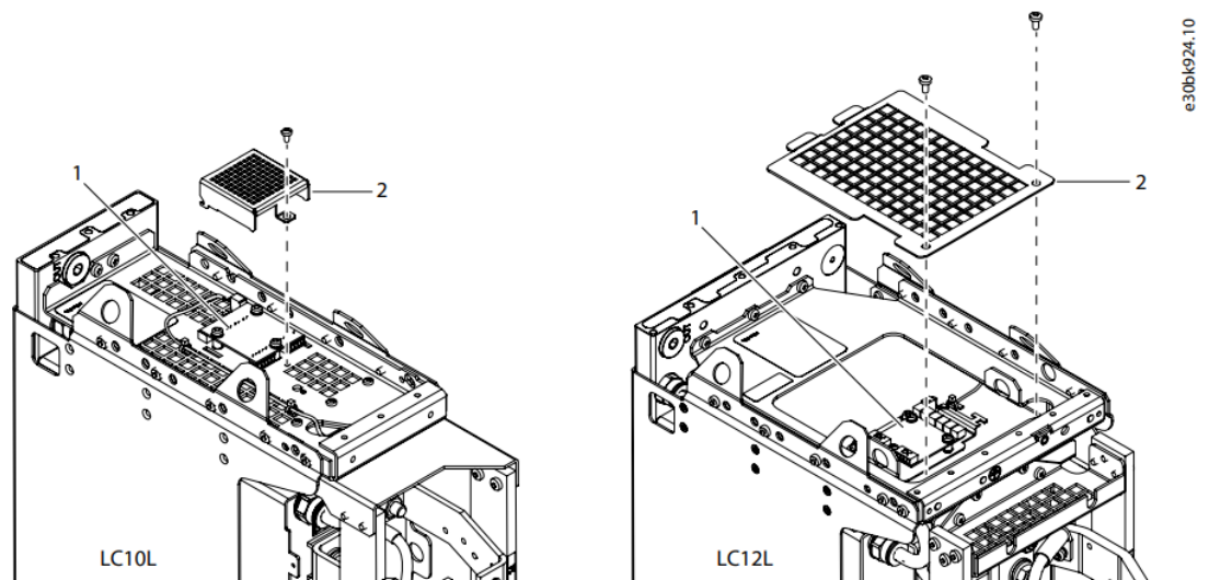
Illustration 12: Accessing the AuxBus Temperature Measurement Board
