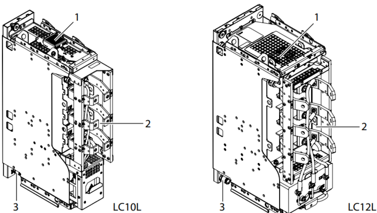
Illustration 1: Liquid-cooled LC Filters
