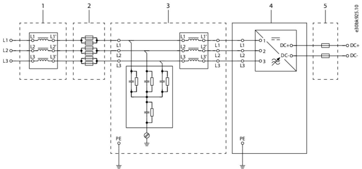
Illustration 16: Wiring Diagram, LC10L
