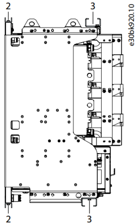
Illustration 3: Example of Mounting the LC Filter in the Cabinet Vertically
