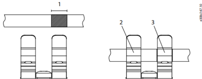
Illustration 15: Using the Cable Clamps
