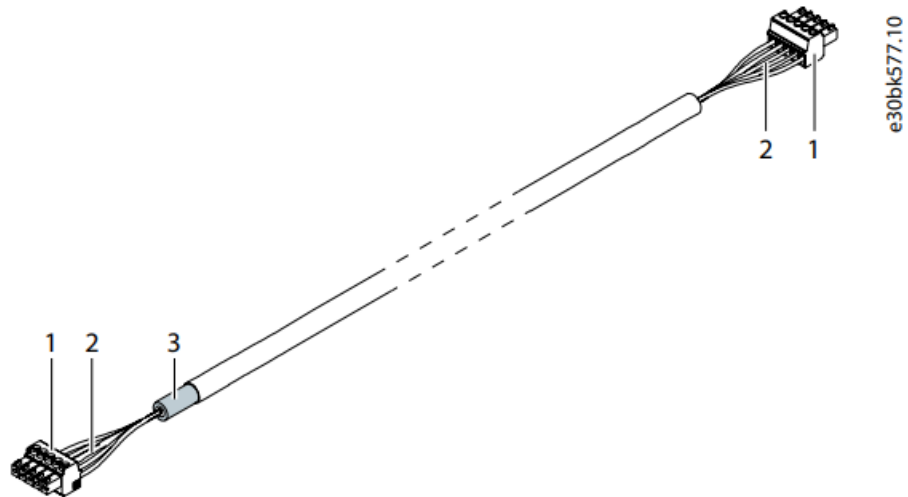
Illustration 11: The Ready AuxBus Cable
