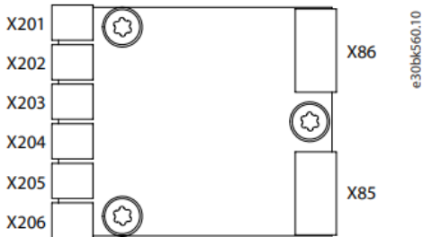
Illustration 13: Terminals on the AuxBus Temperature Measurement Board
