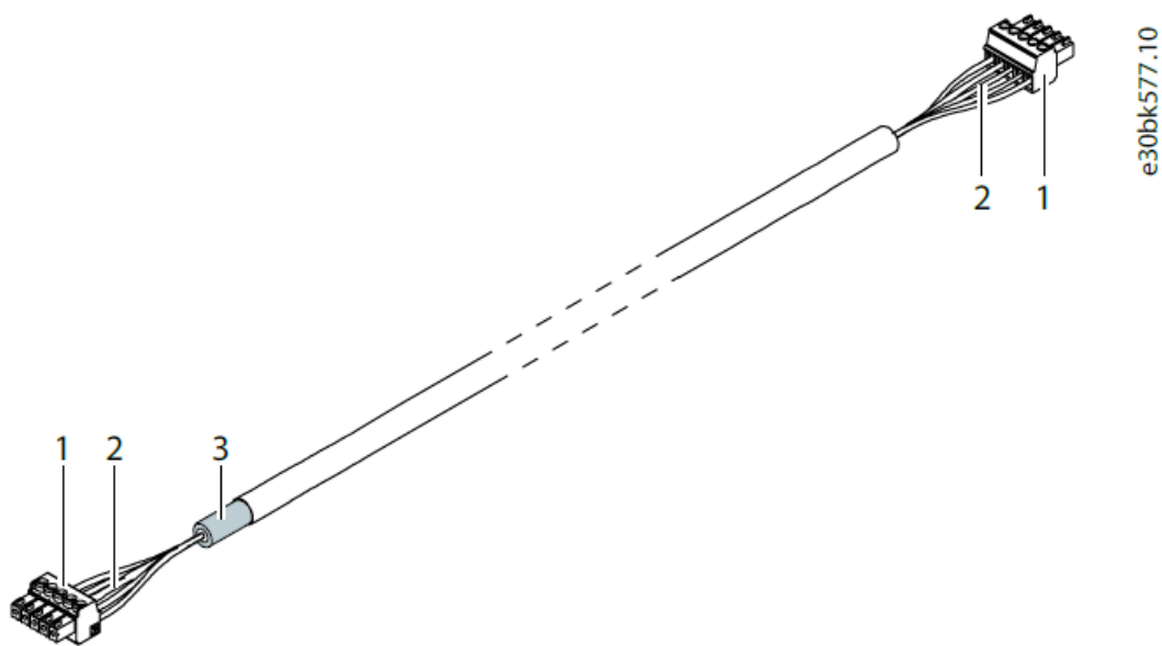
Illustration 11: The Ready AuxBus Cable
