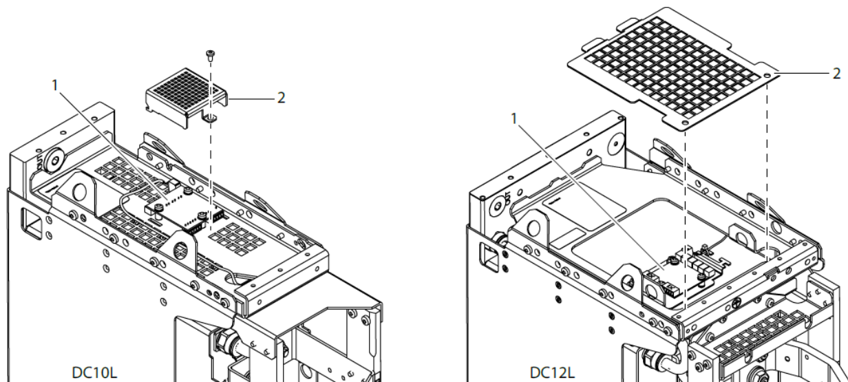
Illustration 12: Accessing the AuxBus Temperature Measurement Board
