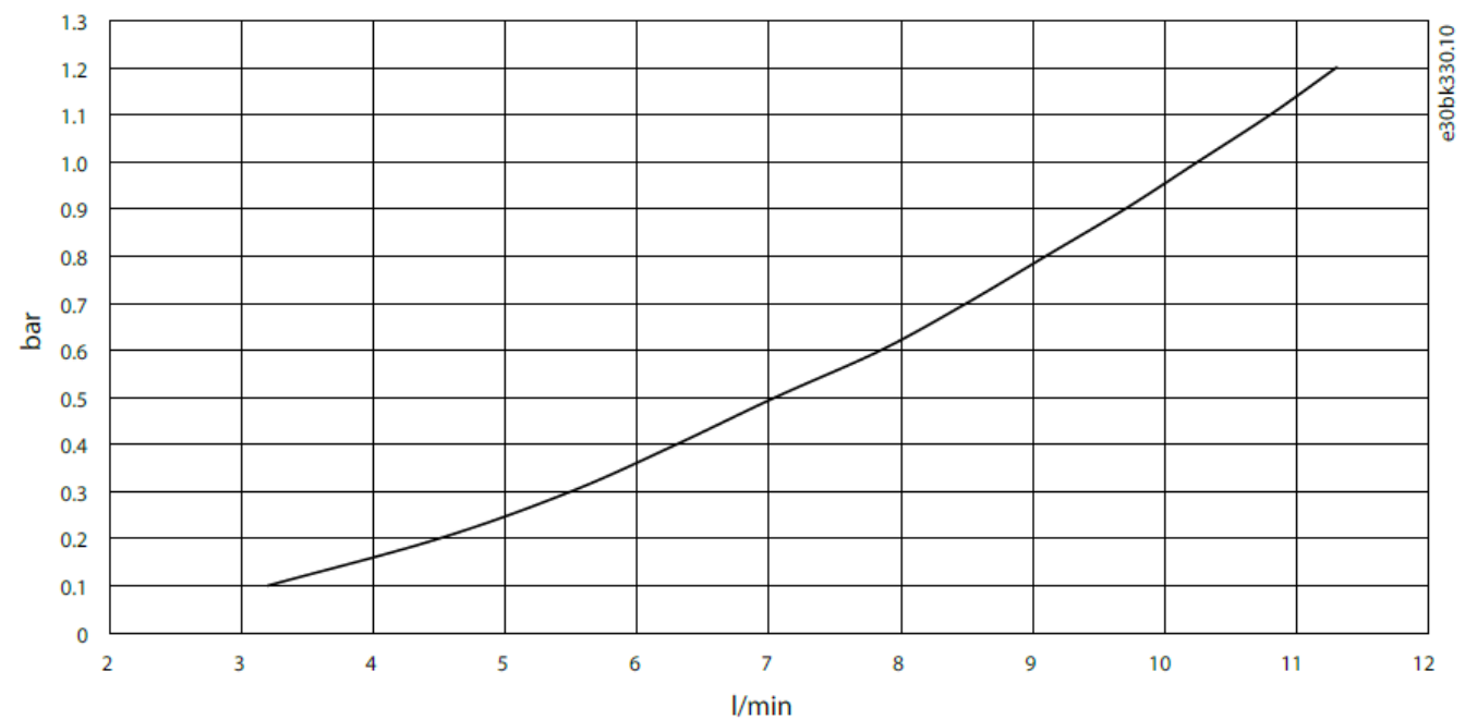
Illustration 7: Pressure Drop with Water, DC10L
