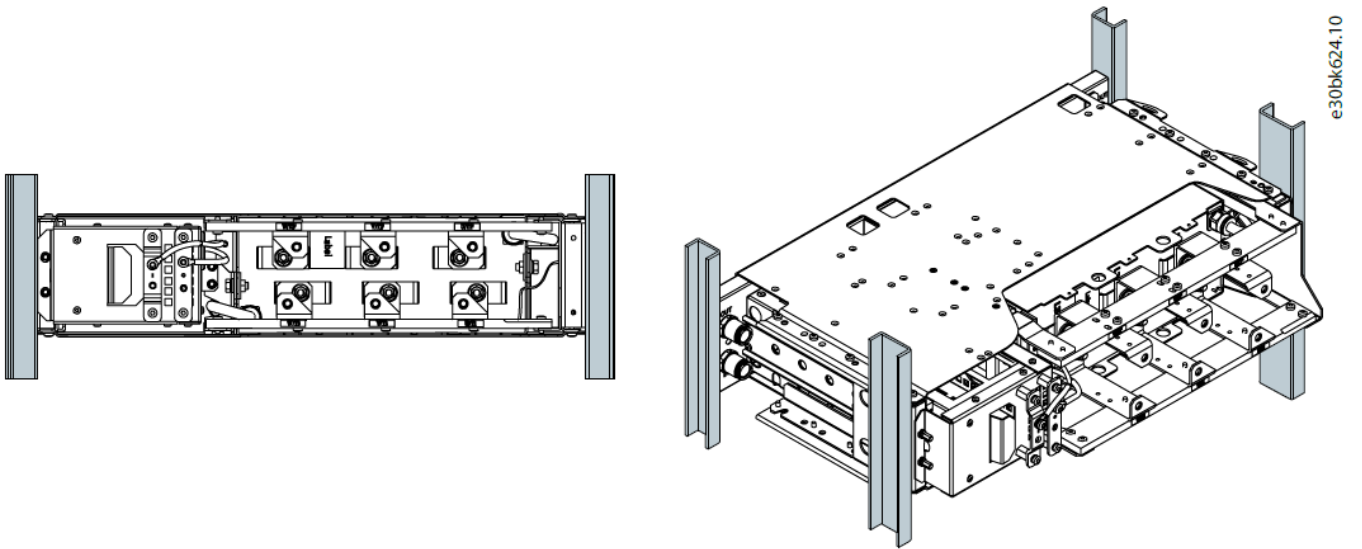
Illustration 4: Example of Mounting the DC Filter Horizontally
