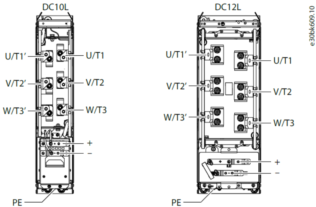
Illustration 10: Terminals of the DC Filter
