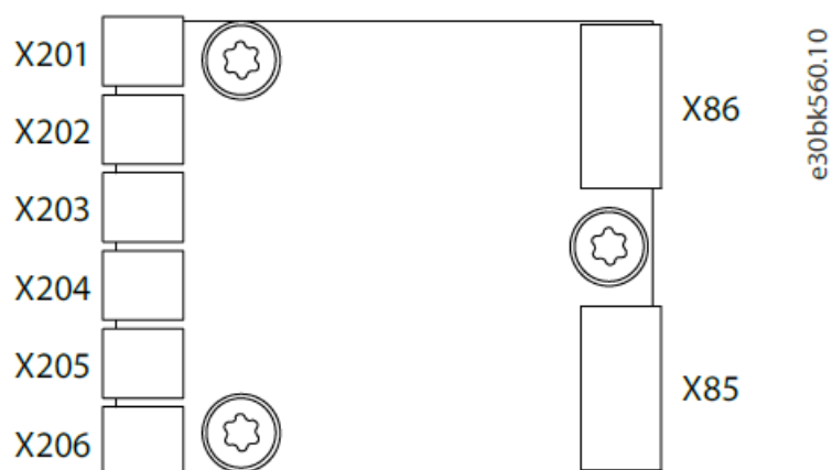
Illustration 13: Terminals on the AuxBus Temperature Measurement Board
