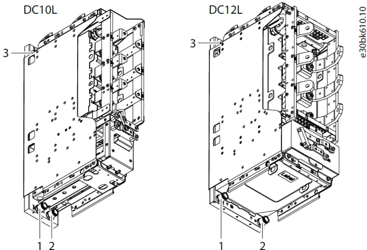
Illustration 9: Location of the Cooling Circuit Connectors
