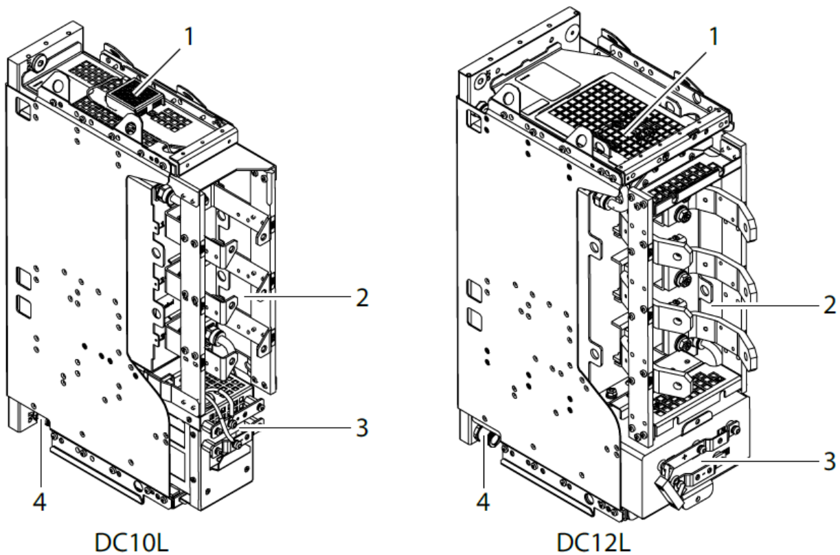
Illustration 1: Liquid-cooled DC Filters
