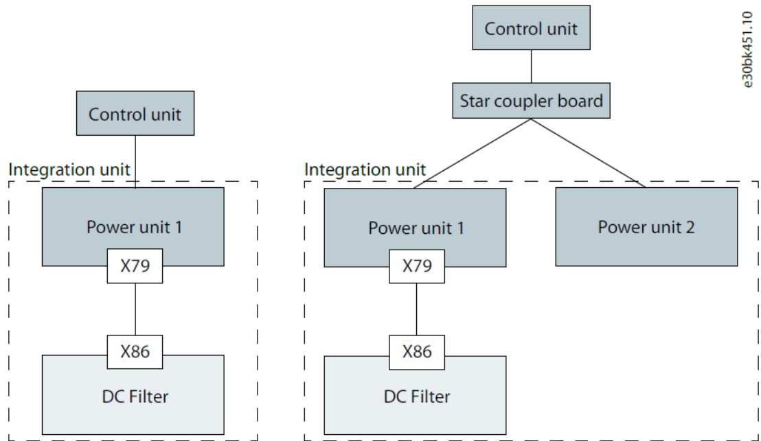
Illustration 14: AuxBus Topology
