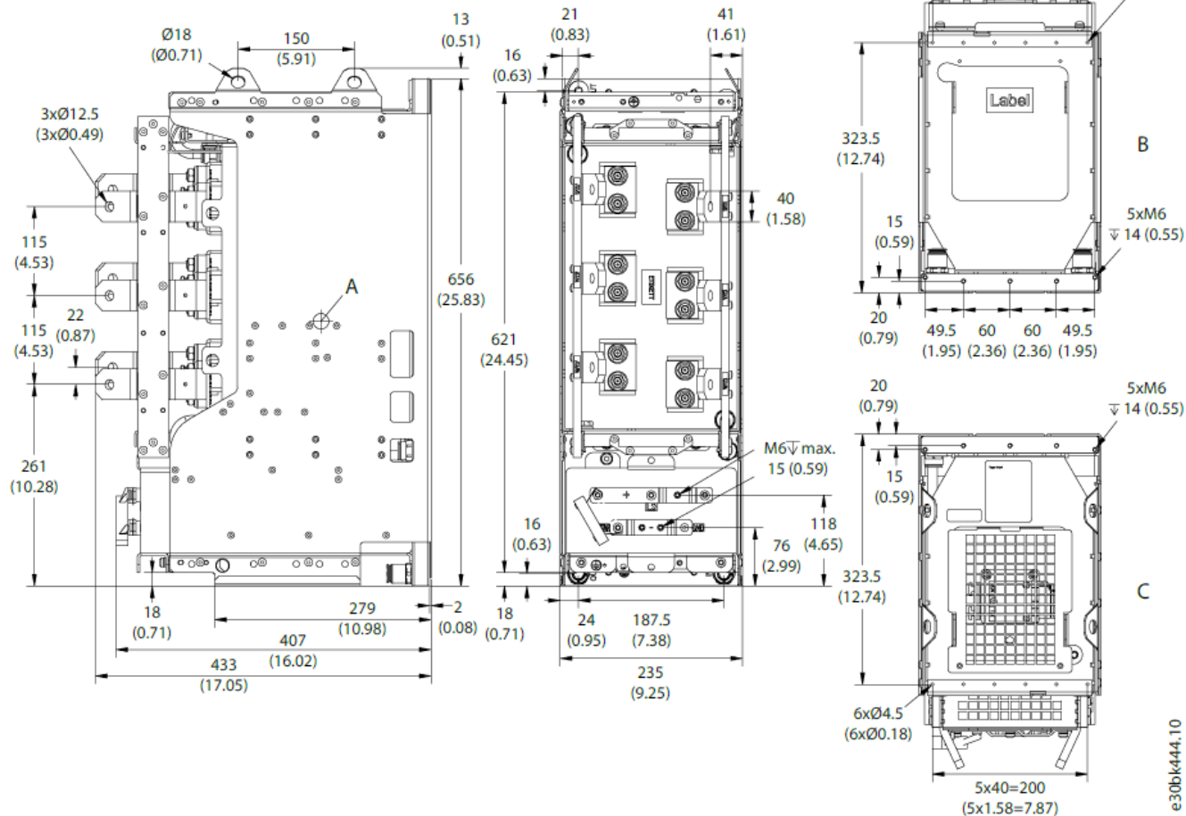
Illustration 6: Dimensions of DC Filter DC12L in mm (in)
