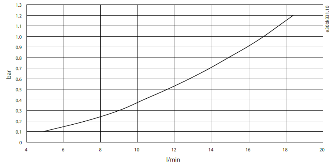
Illustration 8: Pressure Drop with Water, DC12L
