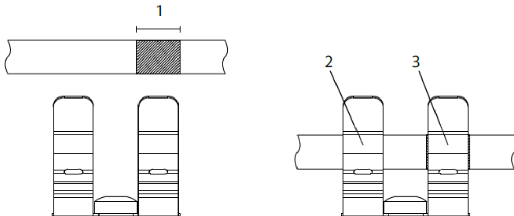
Illustration 15: Using the Cable Clamps
