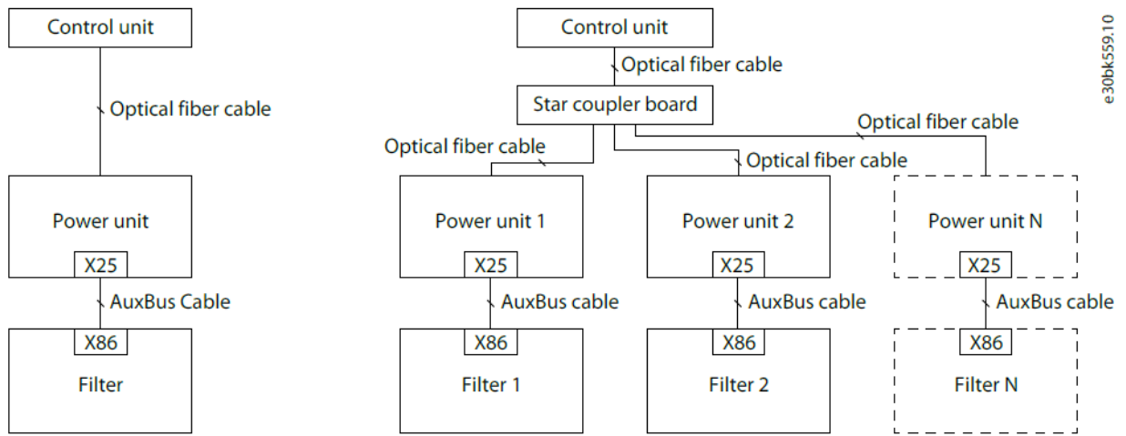
Illustration 14: AuxBus Topology
