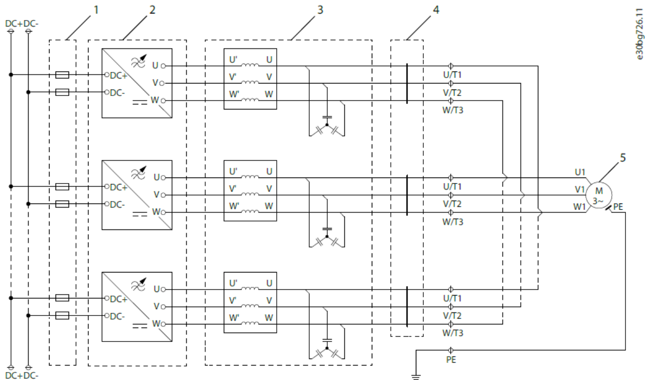
Illustration 17: Wiring Diagram for Inverter with Parallel Power Units and dU/dt Filters
