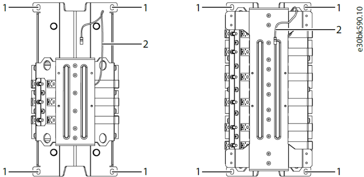
Illustration 2: Mounting Holes of the dU/dt Filter Inductor
