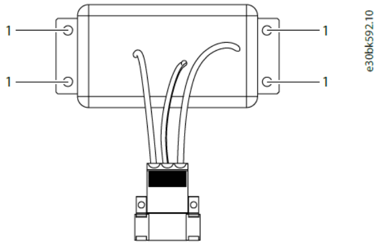
Illustration 4: Mounting Holes of the Capacitor Assembly
