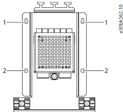
Illustration 5: Mounting Holes of the Assembly Plate
