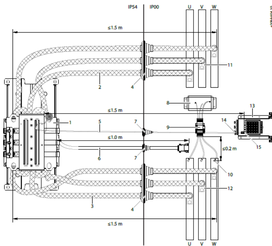
Illustration 11: dU/dt Filter Cable Connections
