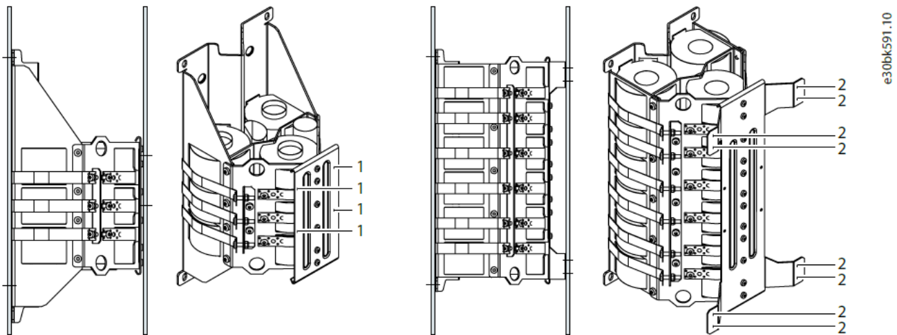
Illustration 3: Mounting Holes on the Front Support Plate of the Inductor
