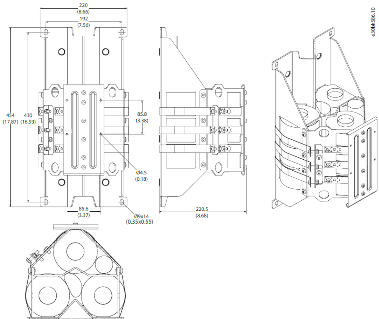
Illustration 7: Dimensions of the dU/dt Filter 590 A Inductor in mm (in)
