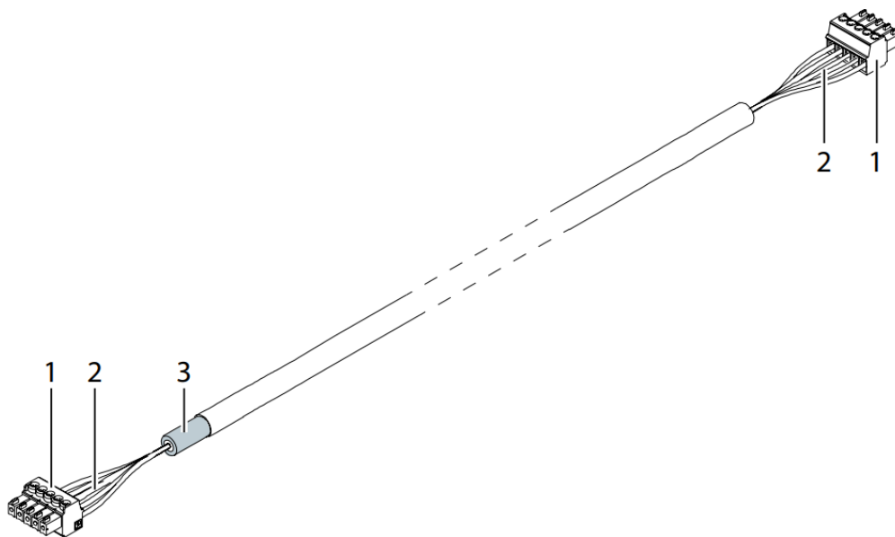
Illustration 12: The Ready AuxBus Cable
