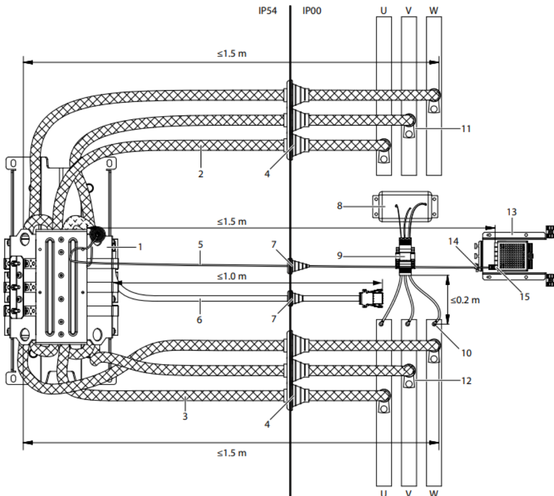
Illustration 11: dU/dt Filter Cable Connections
