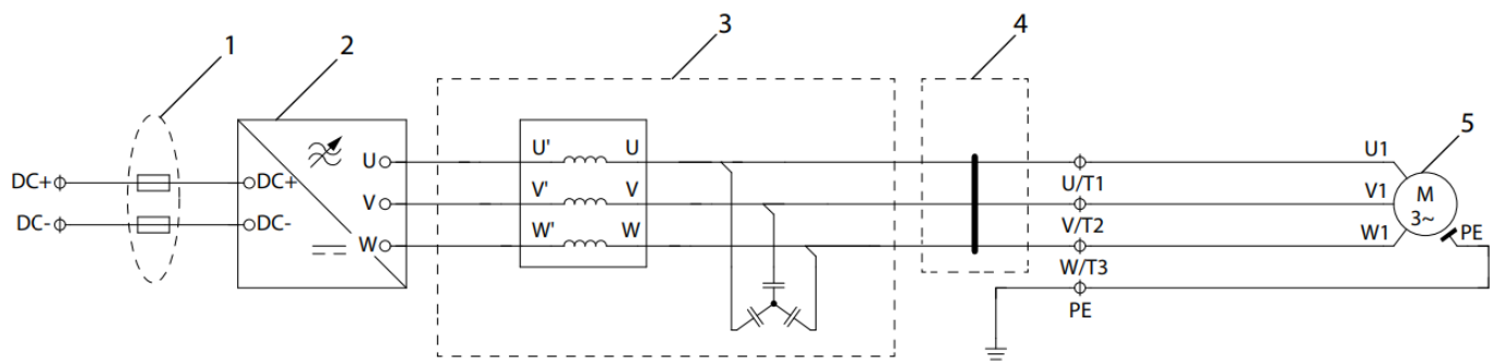
Illustration 16: Wiring Diagram for Inverter and dU/dt Filter
