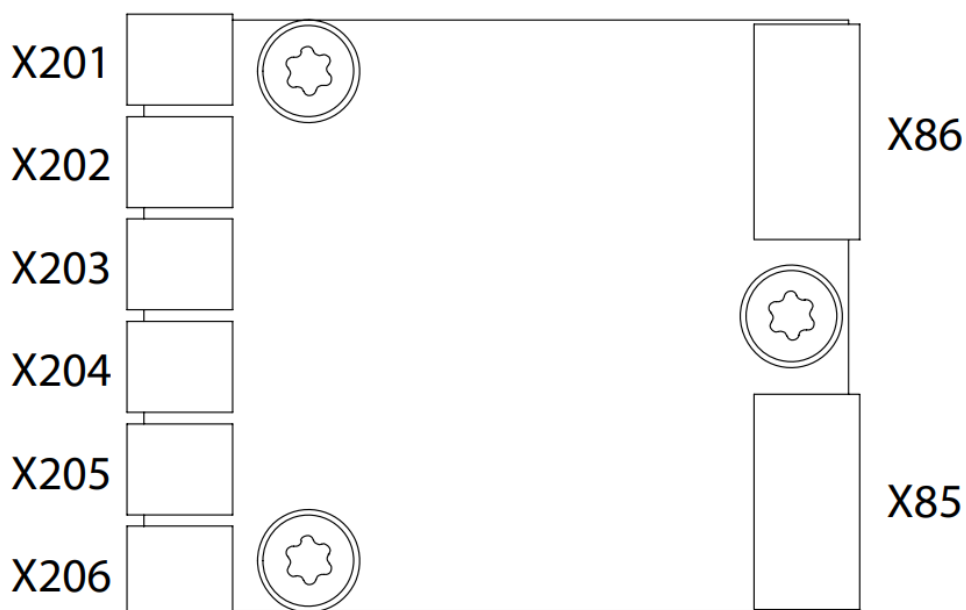
Illustration 13: Terminals on the AuxBus Temperature Measurement Board
