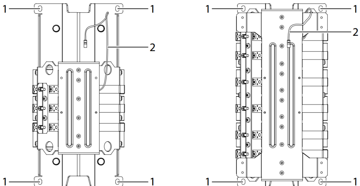
Illustration 2: Mounting Holes of the dU/dt Filter Inductor
