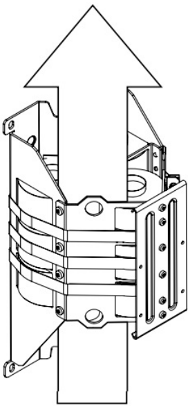
Illustration 6: Air Flow Through the Filter
