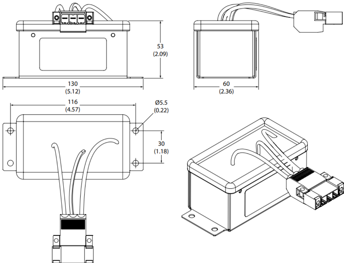
Illustration 10: Dimensions of the dU/dt Filter Capacitor Assembly in mm (in)
