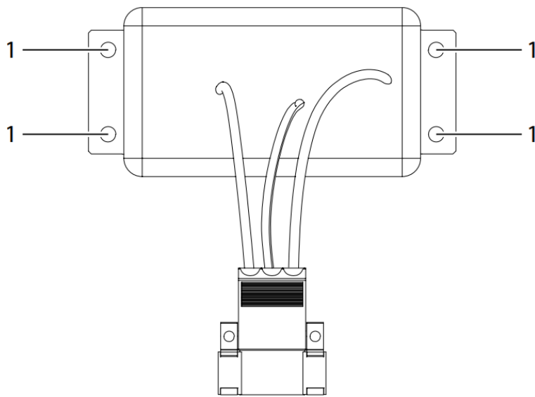
Illustration 4: Mounting Holes of the Capacitor Assembly
