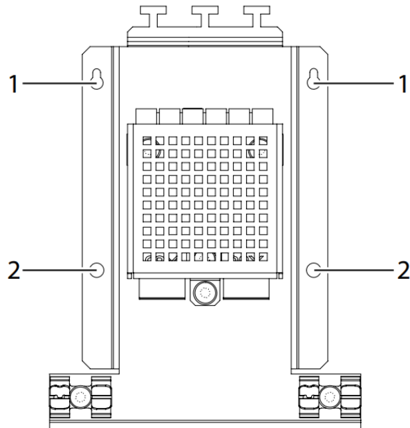
Illustration 5: Mounting Holes of the Assembly Plate
