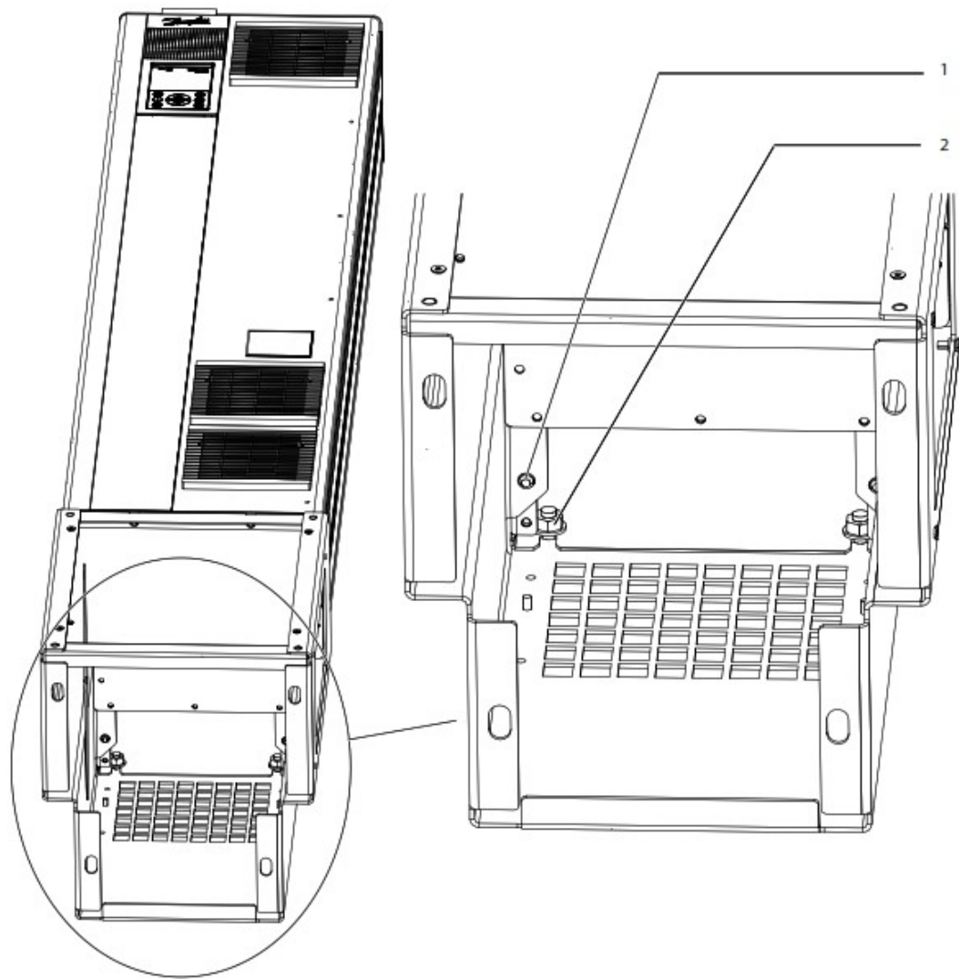
Illustration 3: Pedestal-to-Frequency Converter Mounting Points
