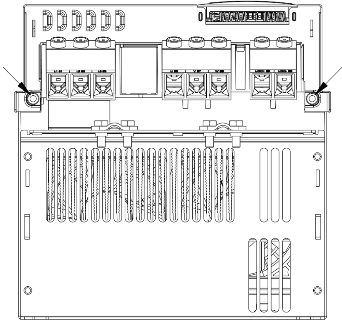
Figure 3: Location of Screws on Base Plate (Taking J6 as an Example)
