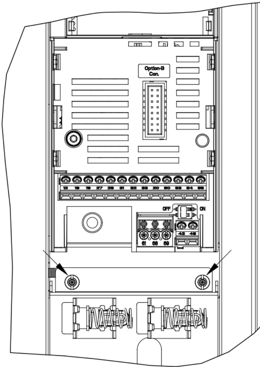
Figure 4: Screws on the I/O Decoupling Plate for Enclosure Size J6
