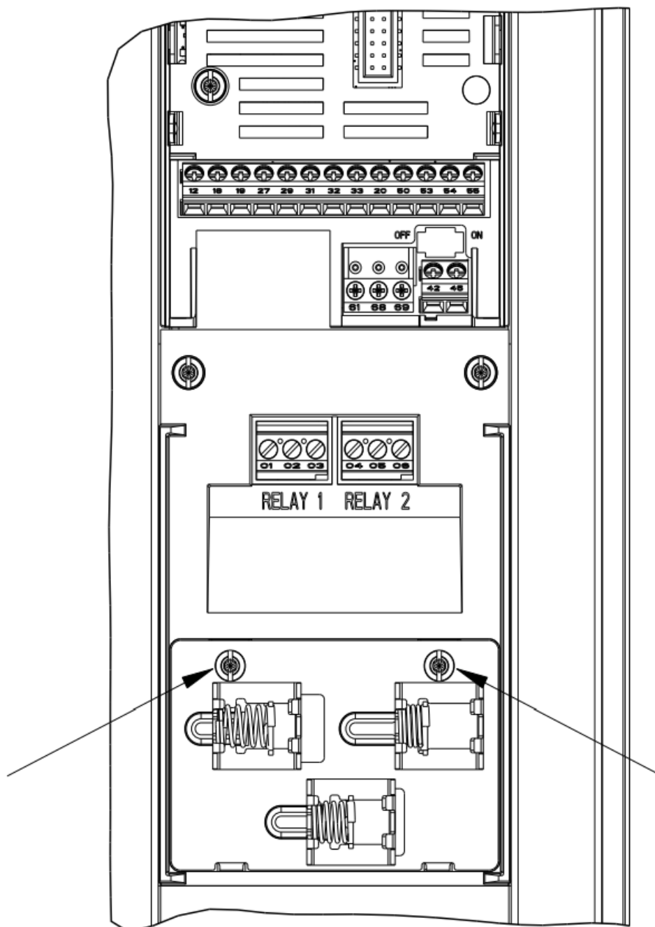
Figure 5: Screws on the I/O Decoupling Plate for Enclosure Size J7
