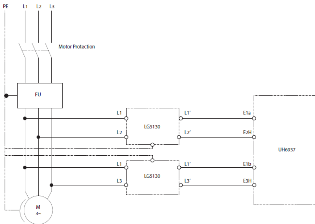
Illustration 3.5 LG 5130 Circuit Diagram
