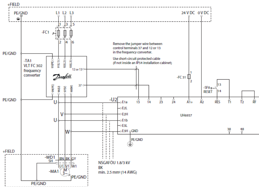
Illustration 3.3 FC 302 and UH 6937 Wiring Diagram
