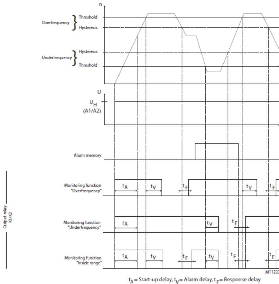
Illustration 3.7 Frequency Monitor Timing
