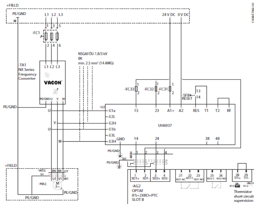
Illustration 3.2 NX Drive, OPT-AF, and UH 6937 Wiring Diagram
