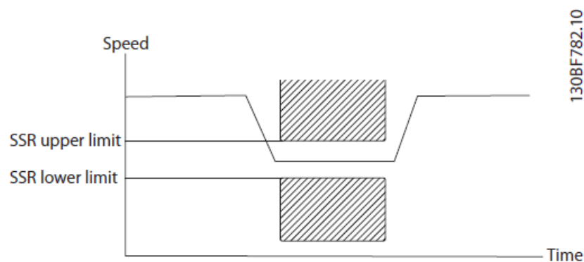
Illustration 2.2 SSR Function
