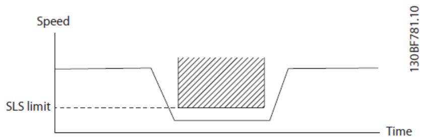
Illustration 2.1 SLS Function
