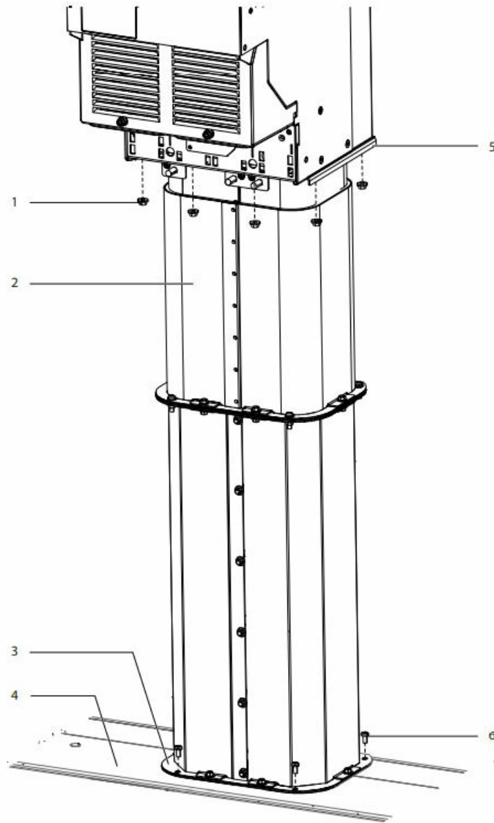
Illustration 13: Installation of the Bottom Duct
