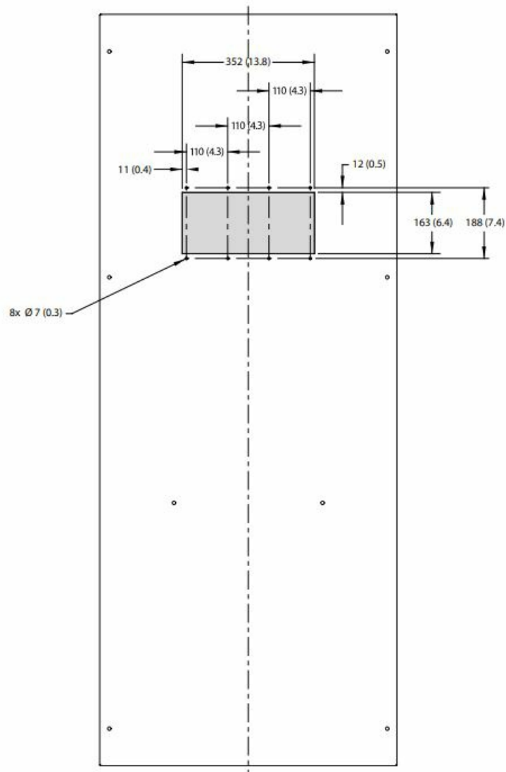
Illustration 6: FA10 Cabinet Backplate Template for In-bottom/Out-back Cooling
