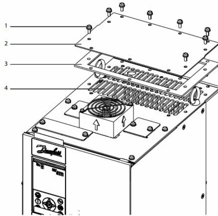
Illustration 7: Installation of the Top Cover
