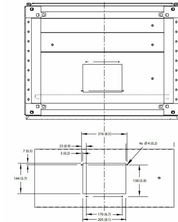
Illustration 8: FA09 Base Plate Template
