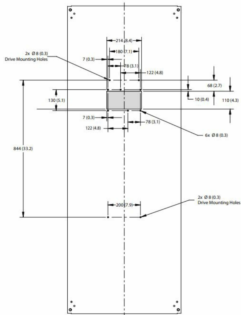
Illustration 3: FA09 Mounting Plate Template for In-bottom/Out-back Cooling
