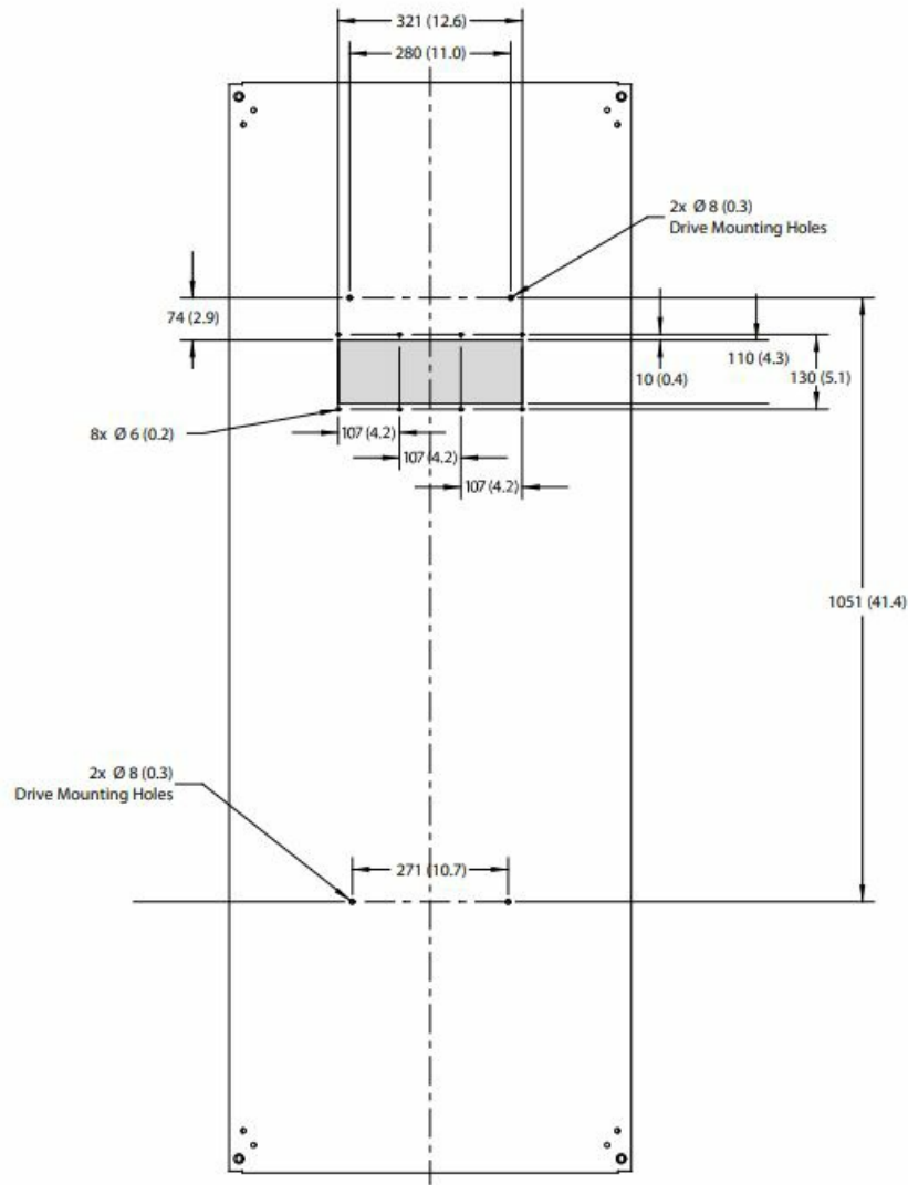
Illustration 4: FA10 Mounting Plate Template for In-bottom/Out-back Cooling
