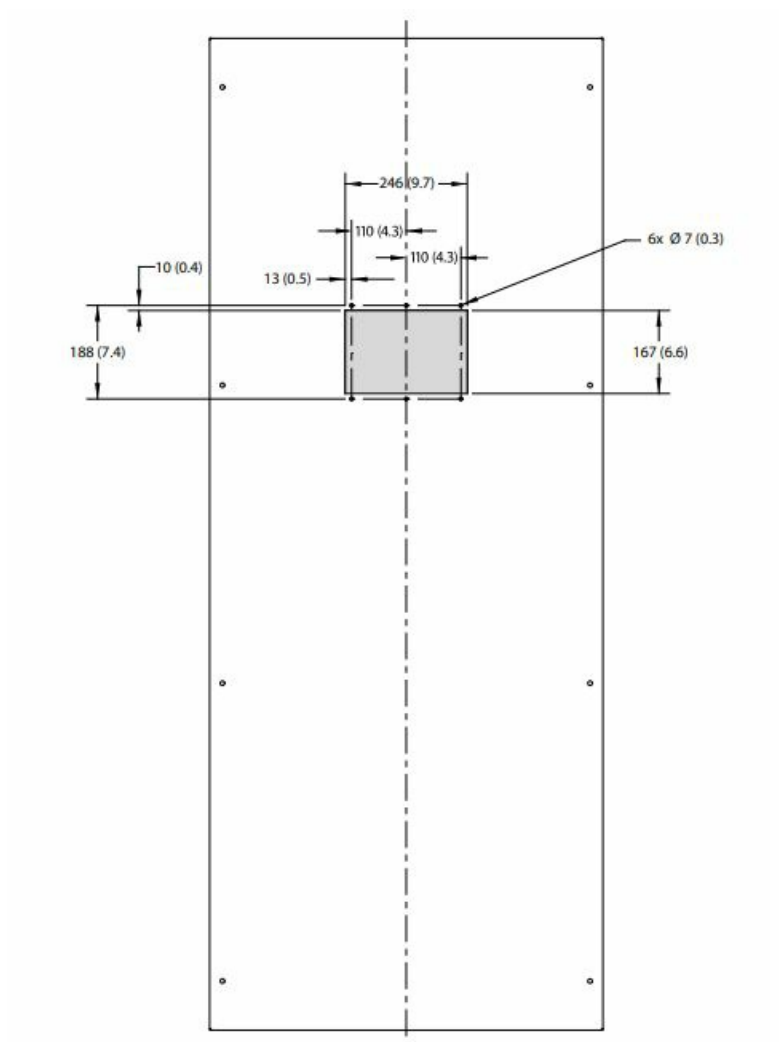
Illustration 5: FA09 Cabinet Backplate Template for In-bottom/Out-back Cooling
