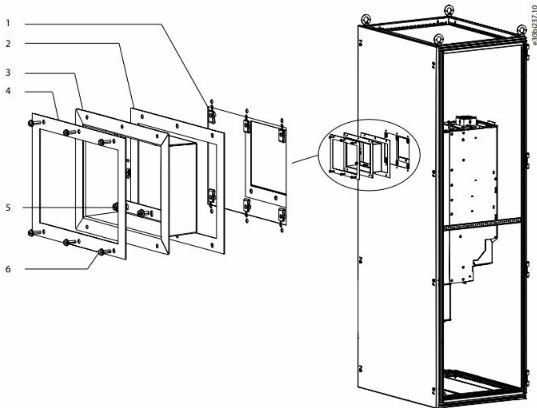
Illustration 14: Installation of Back Vent
