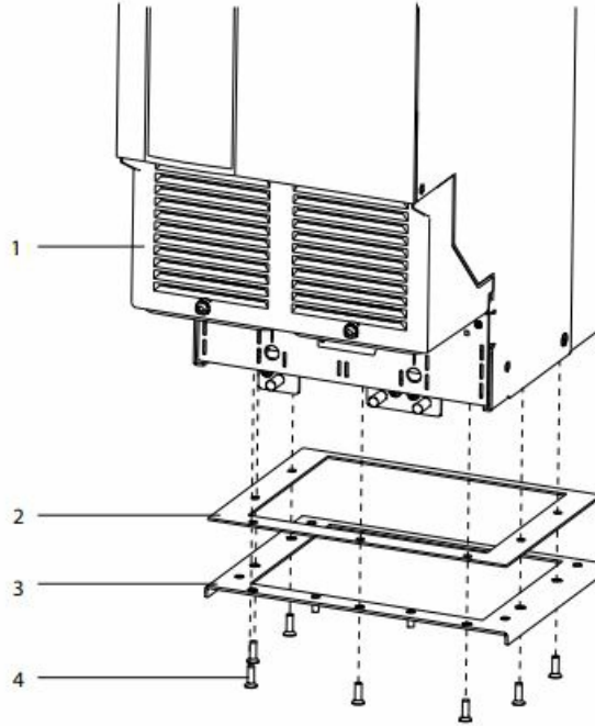
Illustration 11: Installation of the Duct Support Plate
