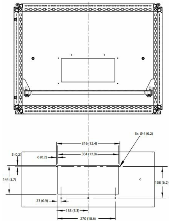
Illustration 8: FA09 Base Plate Template
