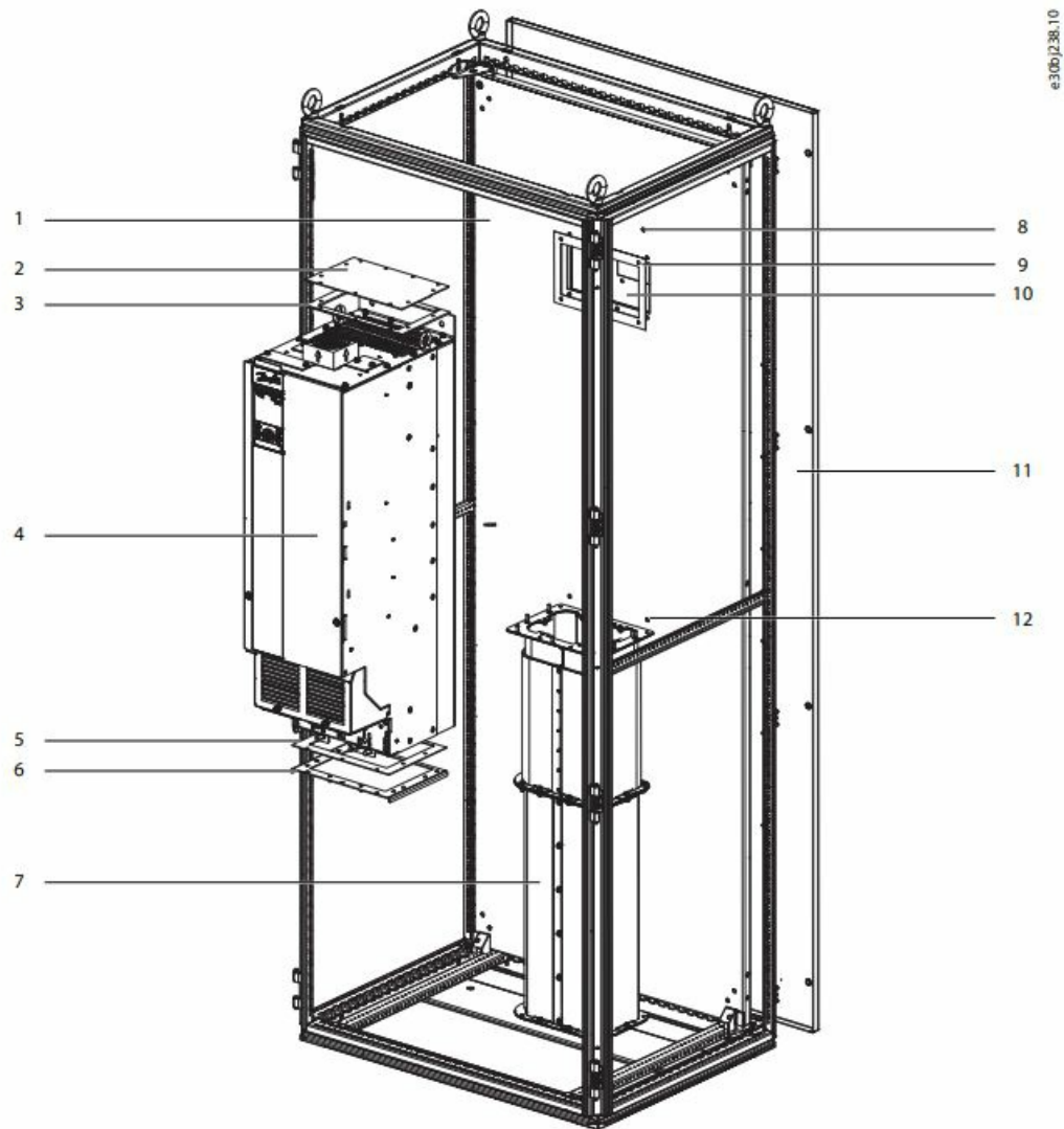
Illustration 2: Overview of In-bottom/Out-back Cooling Kit
