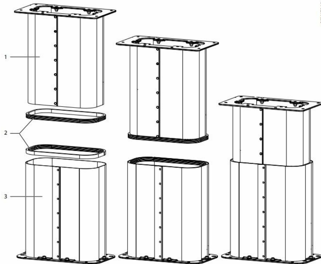
Illustration 12: Assembly of Telescopic Duct
