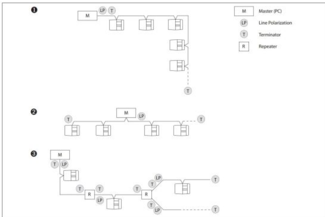
Fig. 4.8a: Daisy chain types
