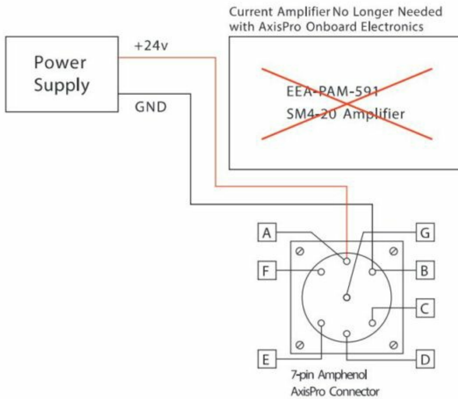
Figure 7. Wiring after mounting the AxisPro valve.
