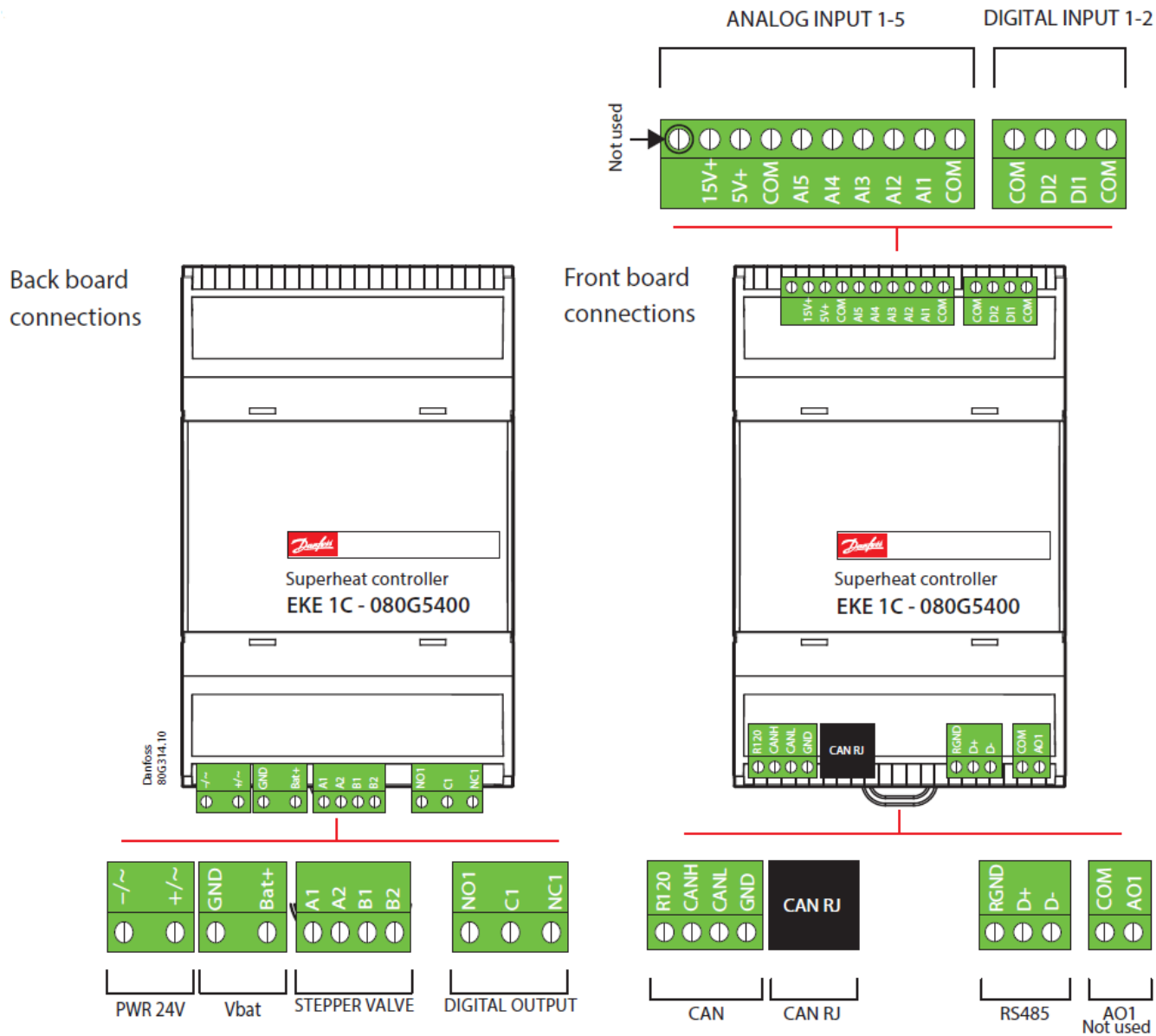
EKE 1C – Front board connection overview
