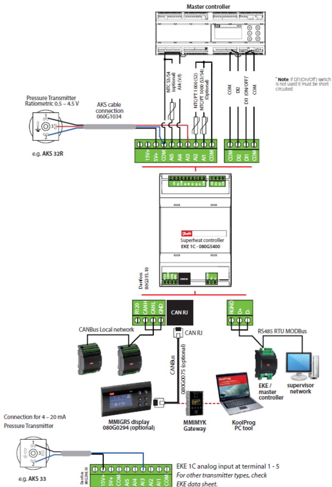
EKE 1C – Back board connection overview
