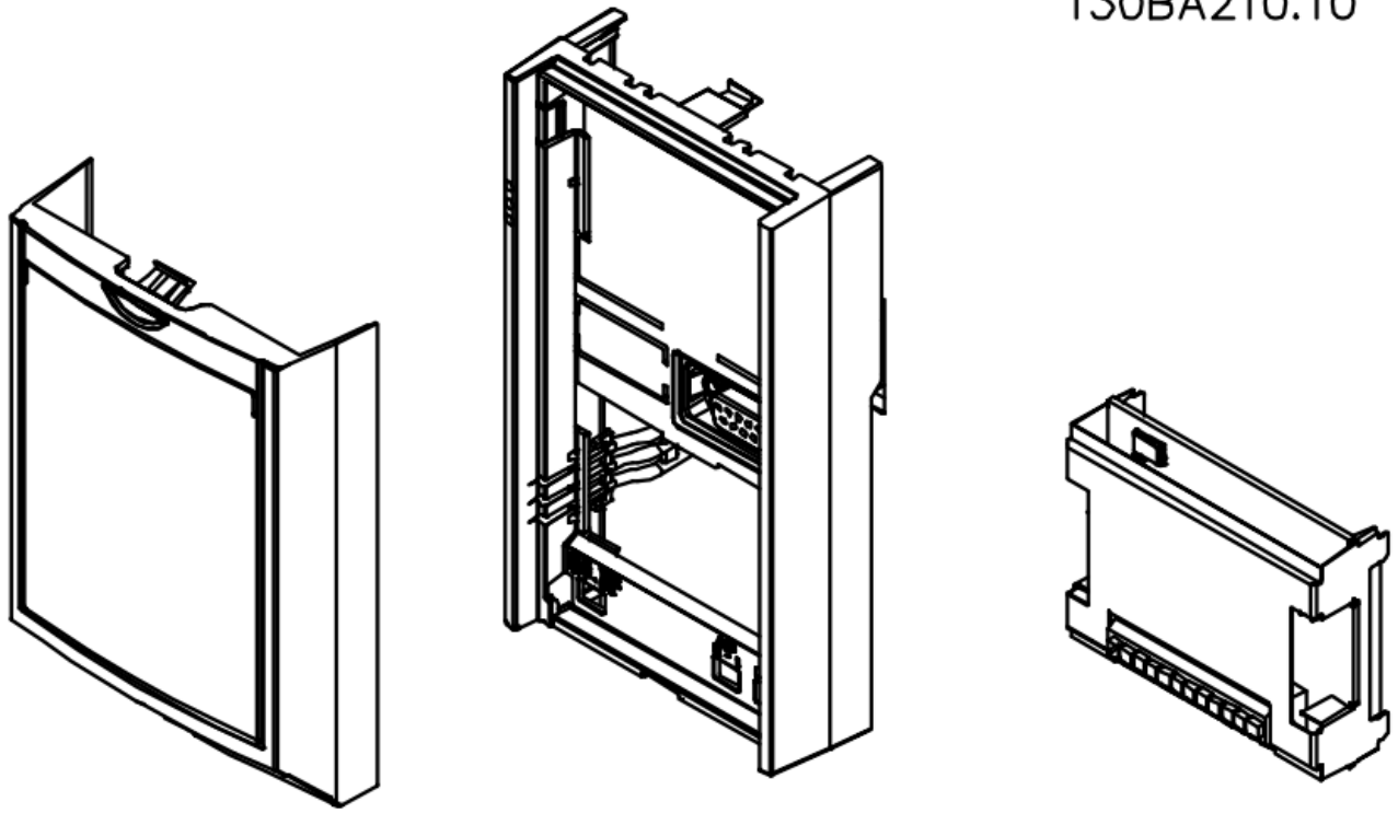
Illustration 1.1 Parts for Coated/Non-coated Code Numbers
