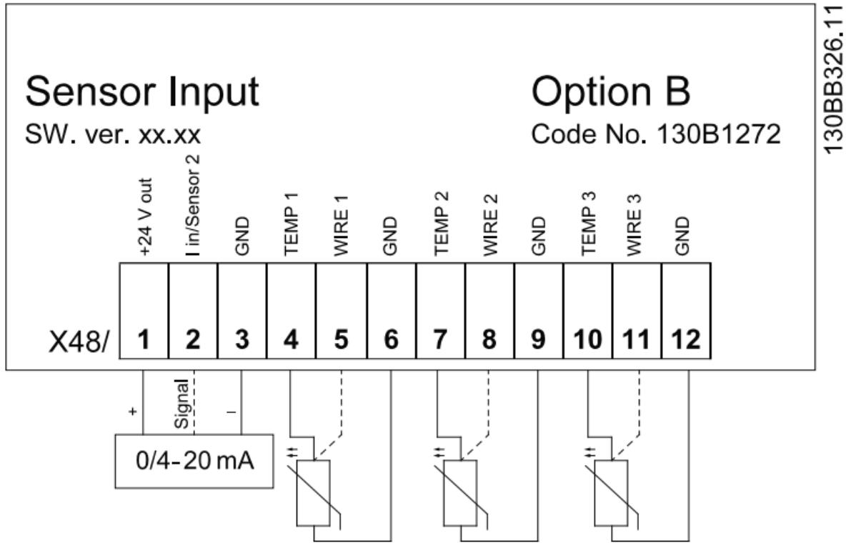
Illustration 1.5 3-Wire Sensors
