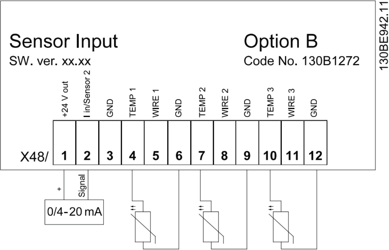
Illustration 1.4 2-Wire Sensors
