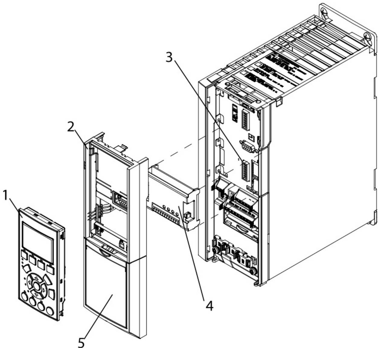
Illustration 1.2 Installation in Enclosure Sizes A2, A3, and B3
