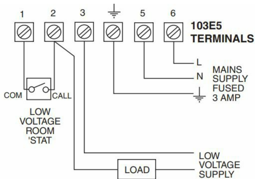
Typical control of Heating when provided by Combination type Boiler
