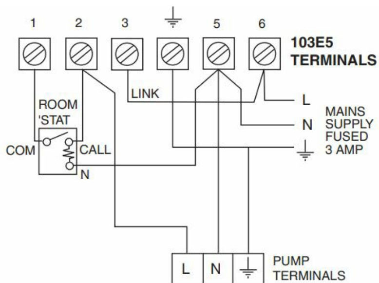
Typical Heating Only system, Boiler and Pump control
