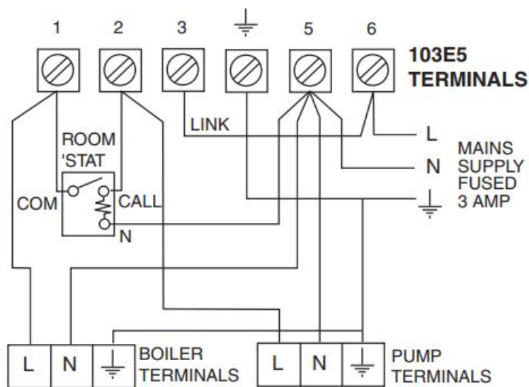
Typical control of Pump for Central Heating on a Solid Fuel System
