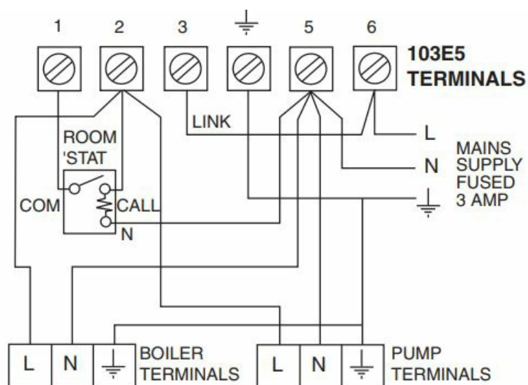
Typical control of Low Voltage System requiring voltage free contacts
