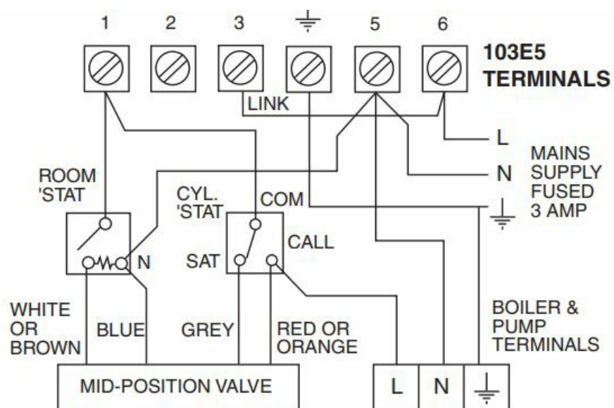
Typical Heating & Hot Water control system using 3 port mid-position valve
