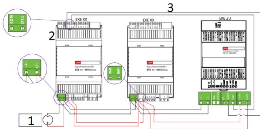
SHARING EKE 2U WITH 2 CONTROLLERS
