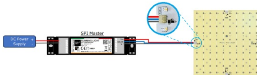
Figure 2: Wiring diagram
