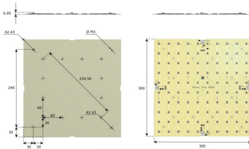
Figure 6: Mechanical dimensions
