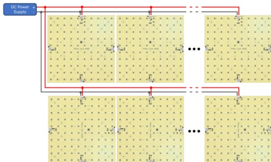
Figure 5: Power Supply, Parallel wiring diagram
