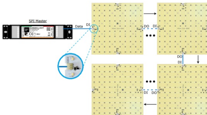
Figure 3: Remote Control Connection Topology, Bus-wiring
