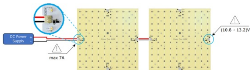
Figure 4: Power Supply, Series wiring diagram
