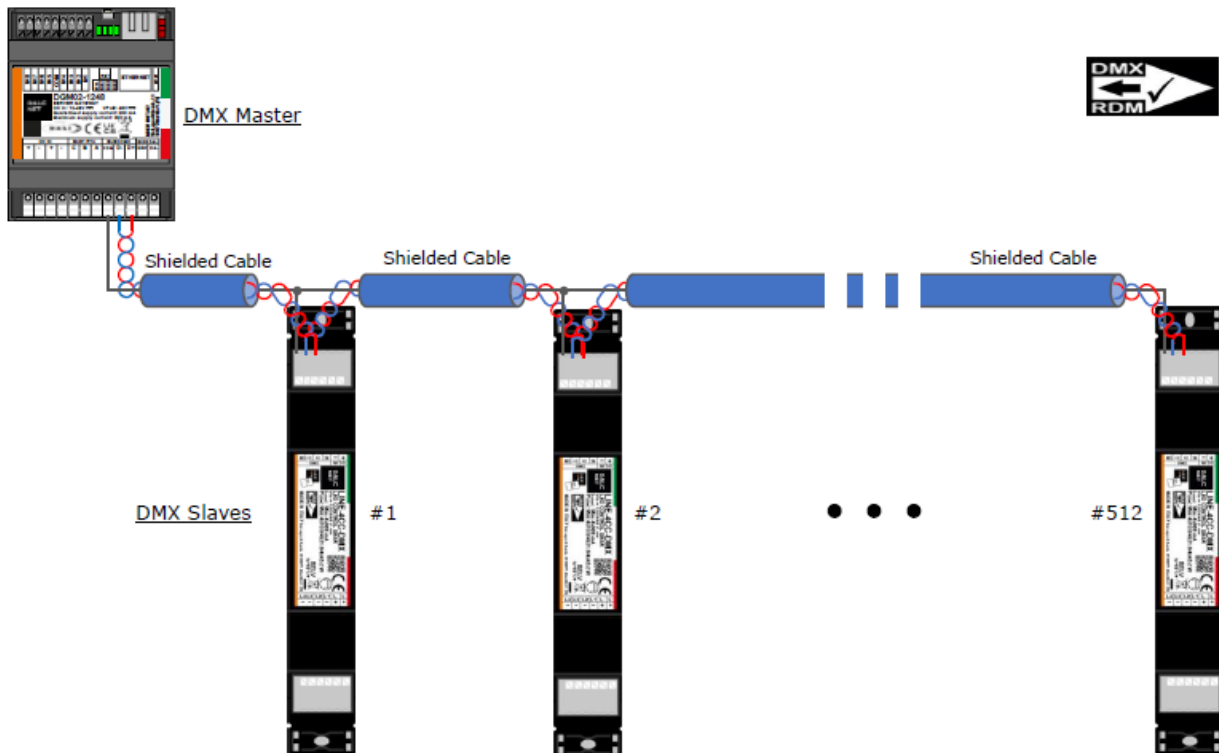
Figure 7: Remote Control Connection Topology, Bus-wiring
