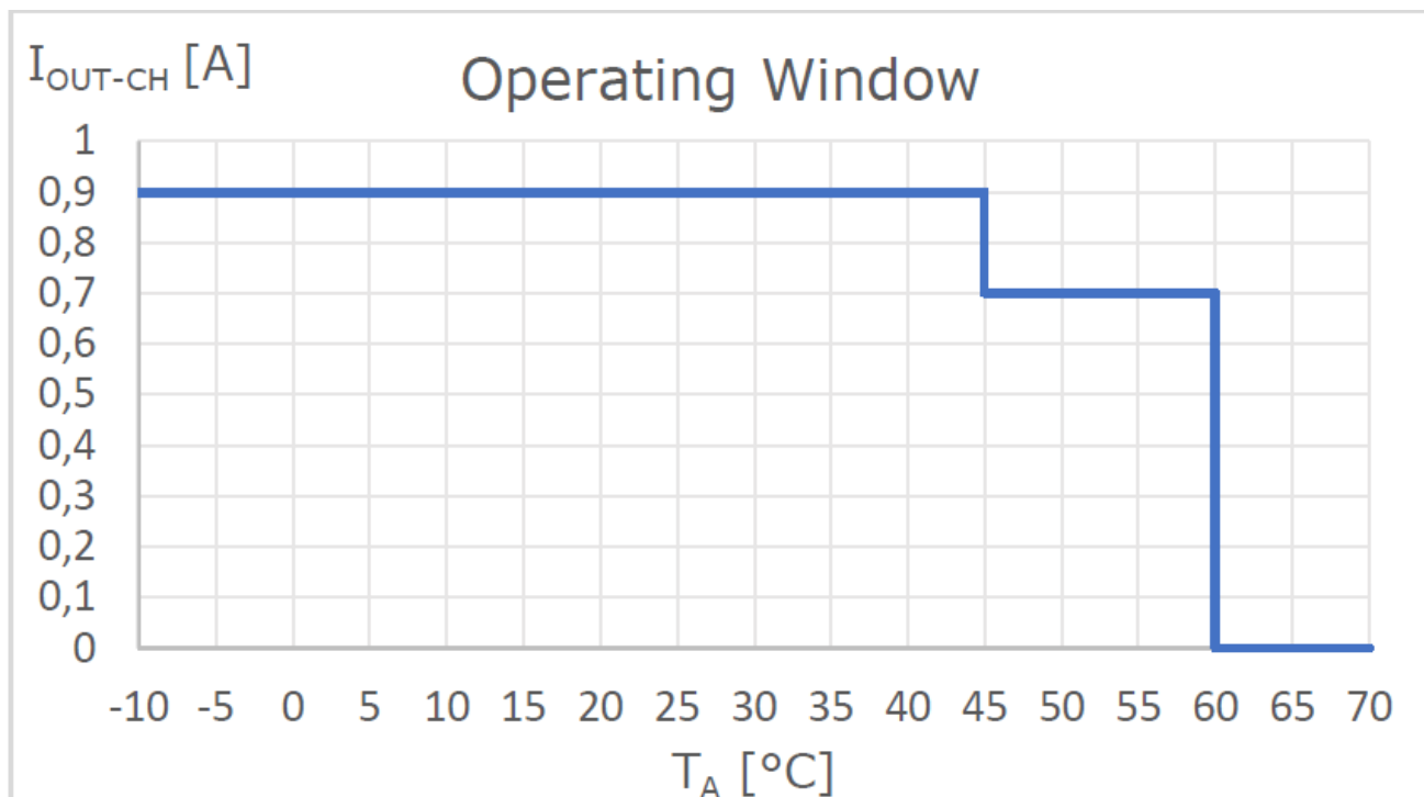
Figure 10: Operating Temperature Window
