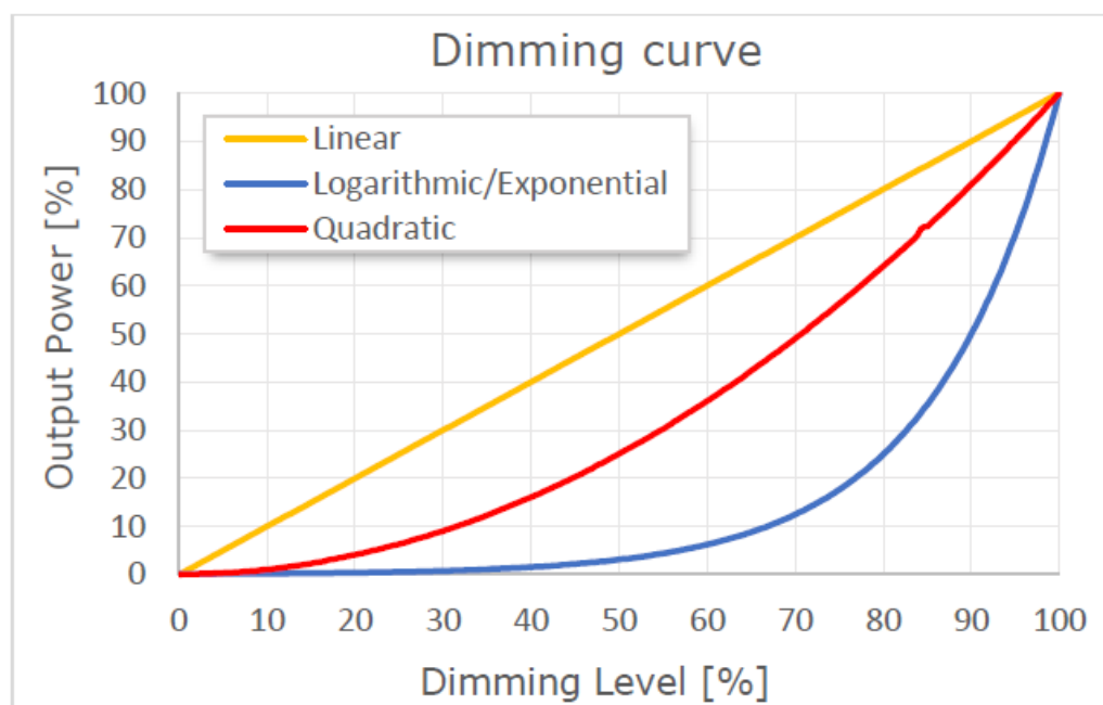
Figure 11: Dimming Curves
