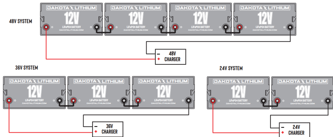
FIG 2: CHARGER LAYOUTS
