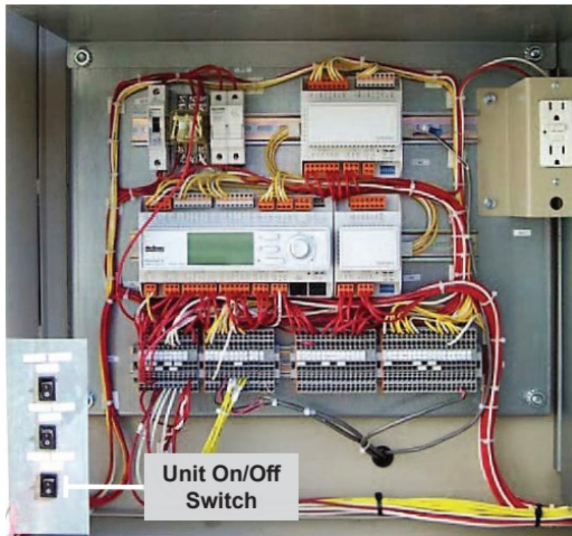
Figure 6: Chiller Unit Controller On/Off Switch
