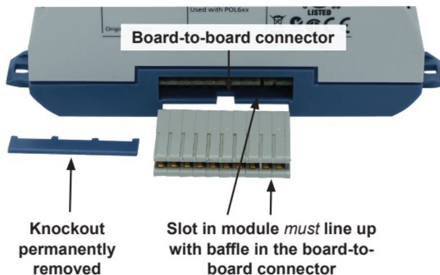
Figure 7: Communication Module and Knockout
