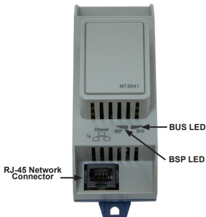
Figure 4: BACnet IP Communication Module
