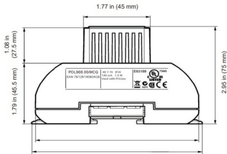
Figure 2: BACnet Communication Module Side View
