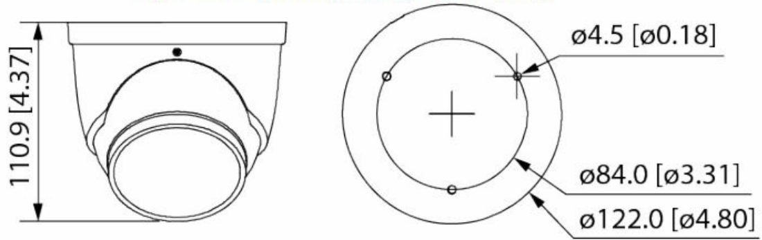
Figure 3-2 Dimensions: Model A (Unit: mm [inch])
