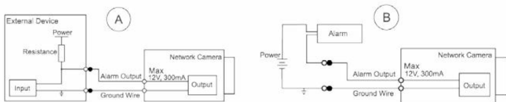
Figure 1-3 Alarm output
