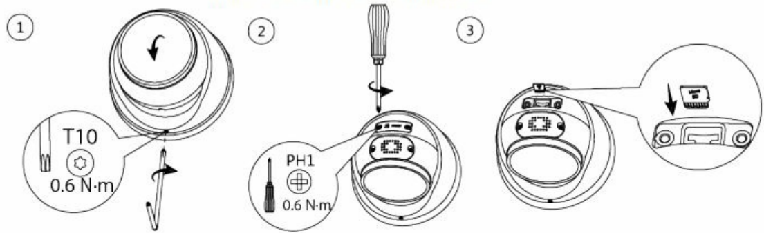
Figure 3-6 Install SD card (Model B)
