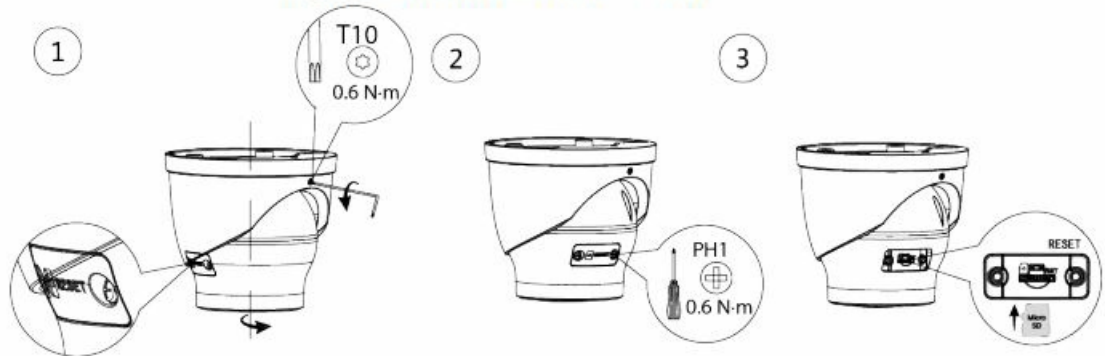
Figure 3-6 Install SD card (Model B)
