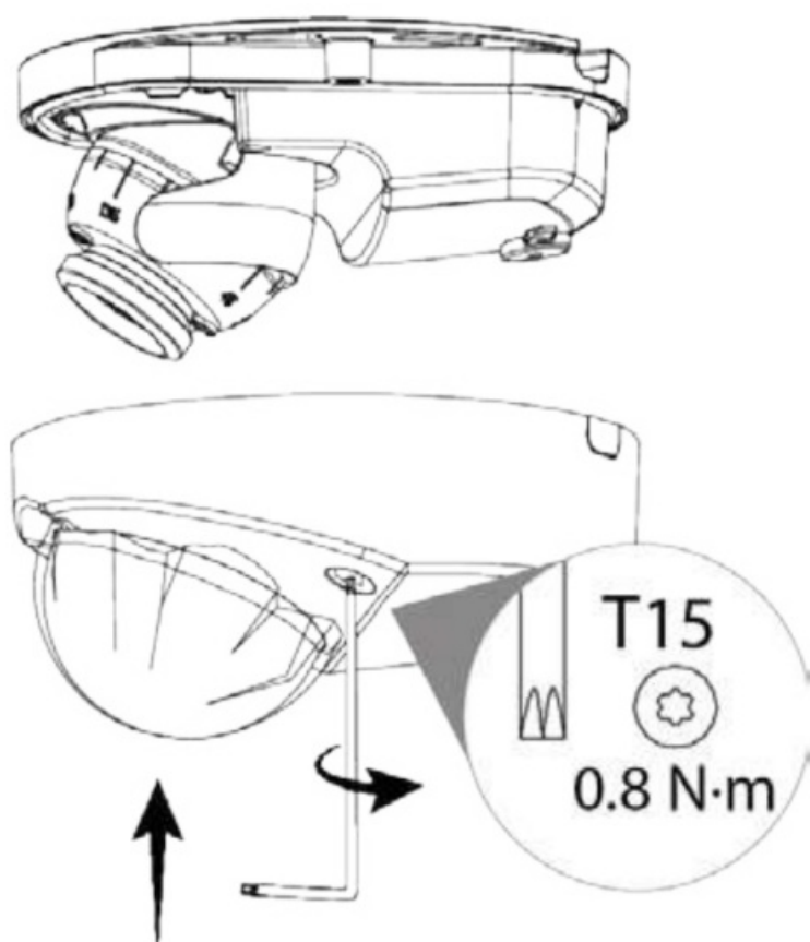
Figure 3-10 Closing the camera
