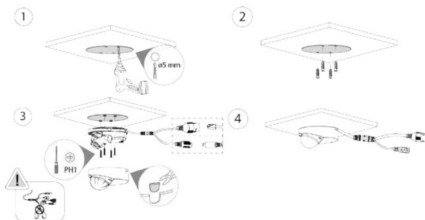
Figure 3-7 Cable going through the mounting surface
