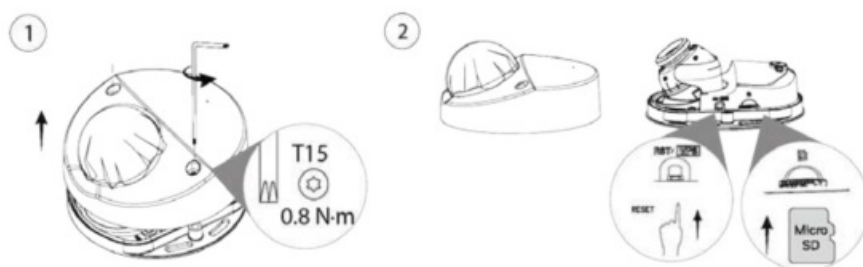
Figure 3-5 Install the SD card
