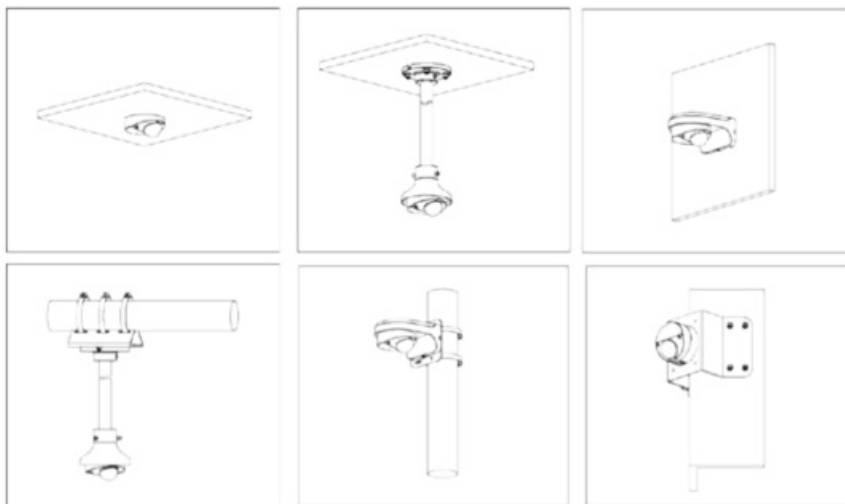
Figure 3-4 Installation methods
