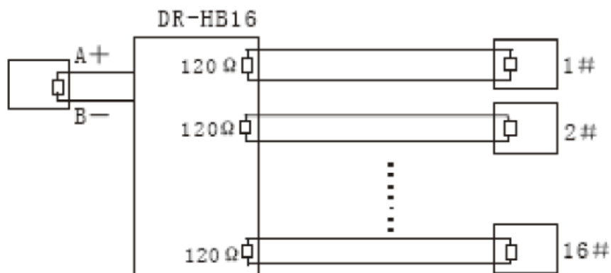
Figure 3-2 Connecting method with RS-485 distributors
