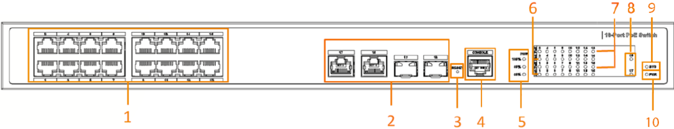
Figure 2-1 Front panel
