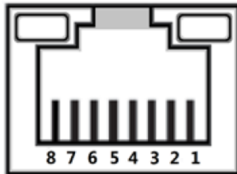
Figure 4-2 Ethernet port pin number
