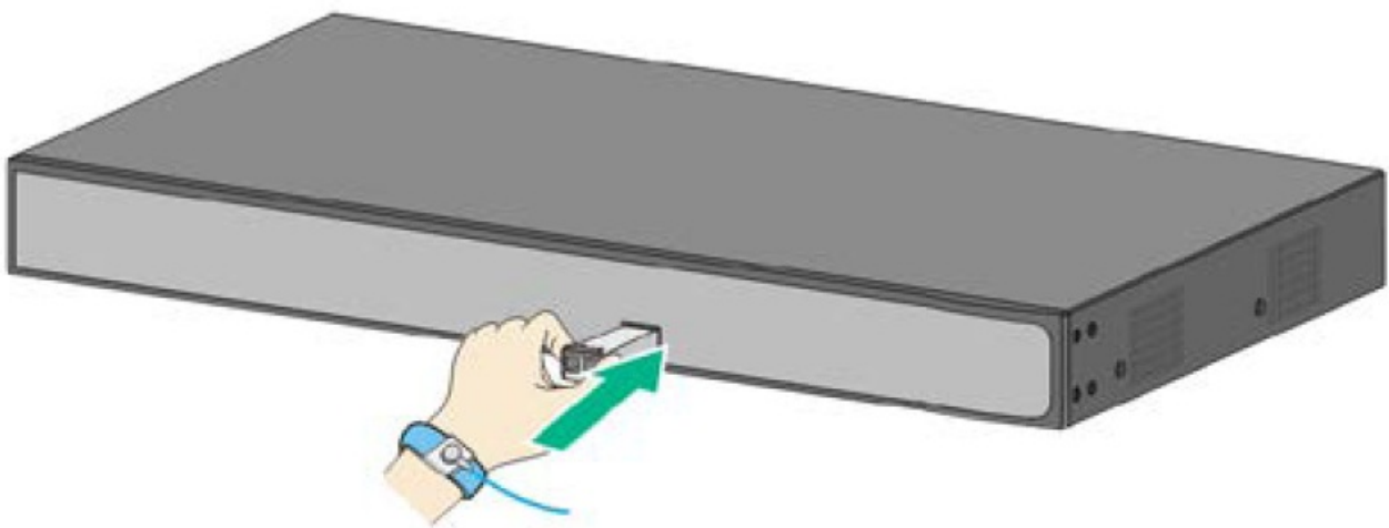
Figure 4-4 Install SFP module
