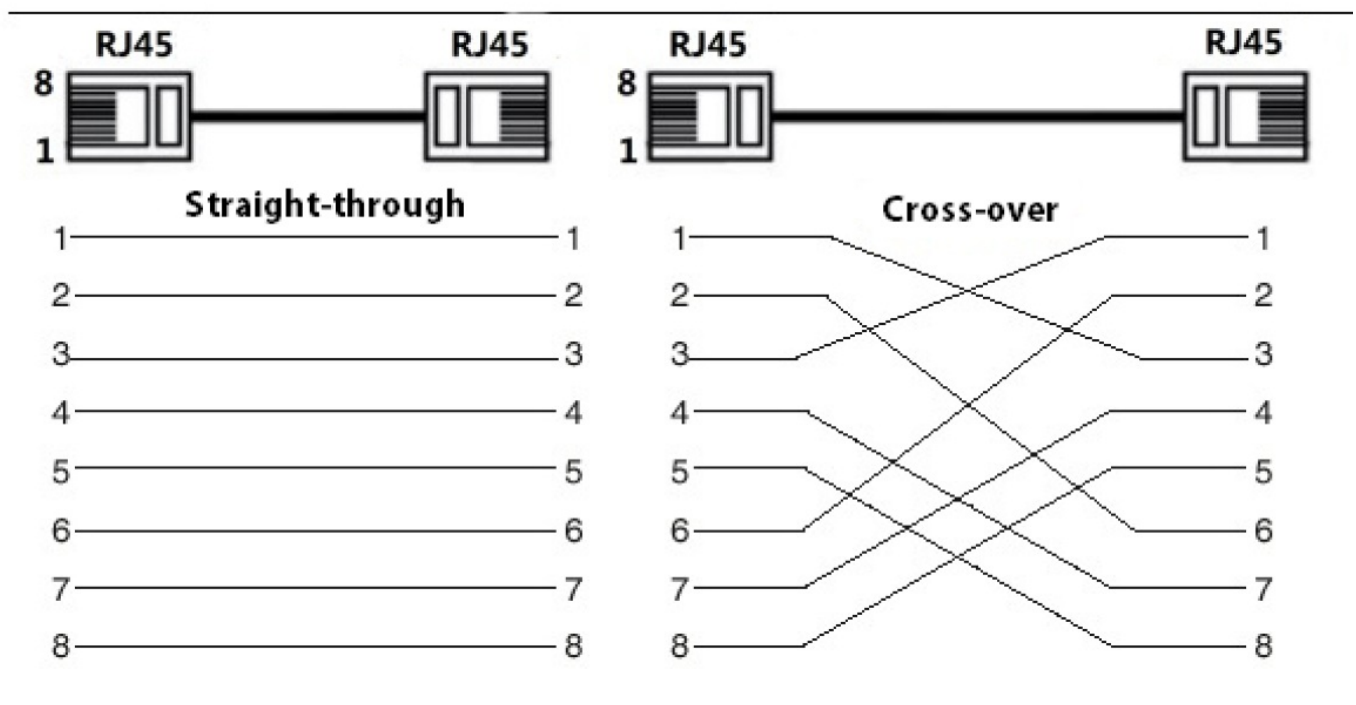
Figure 4-3 Connect cable
