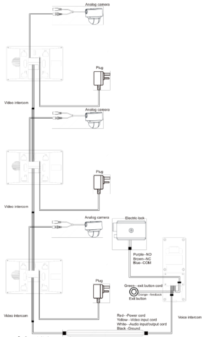
Figure 3-3 Wiring (2)
