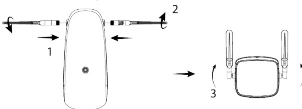
Figure 3-5 Install antennas
