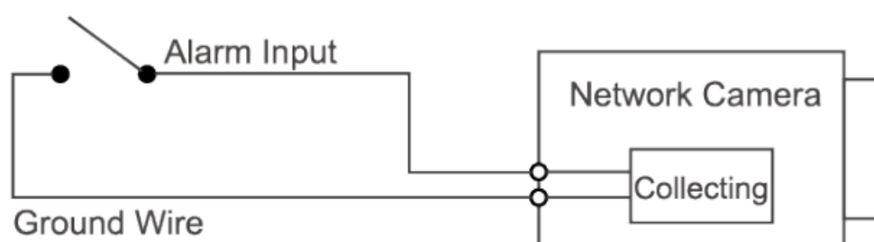
Figure 1-2 Alarm input
