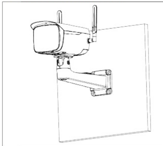
Figure 3-3 Installation method
