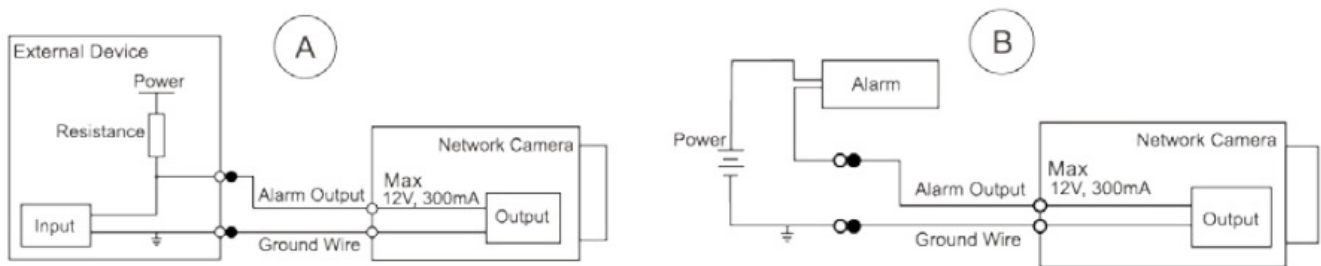
Figure 1-3 Alarm output
