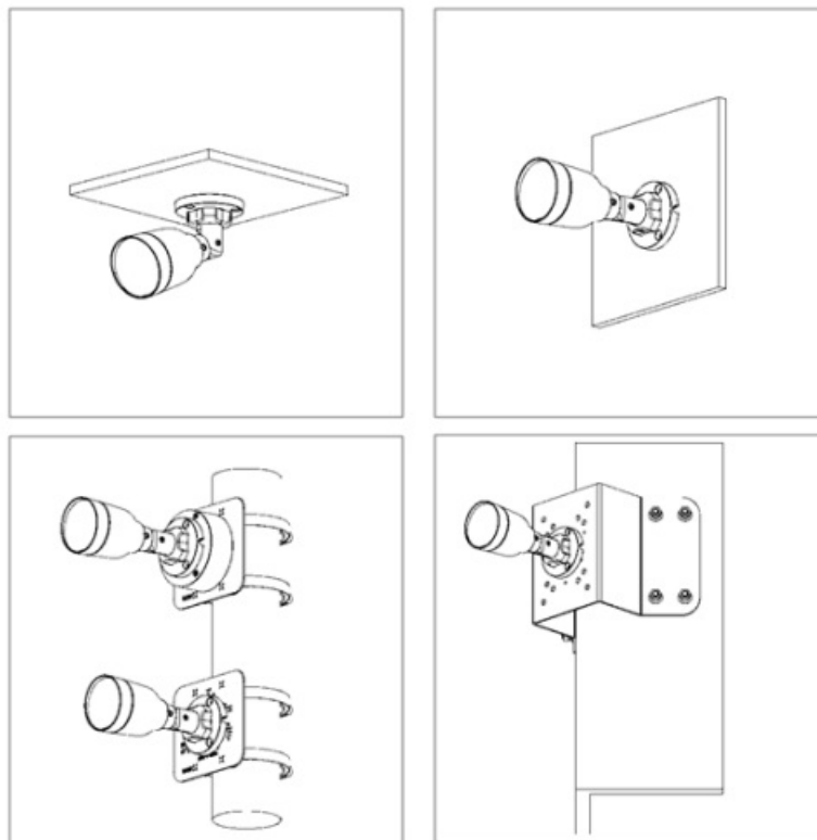
Figure 4-4 Installation methods
