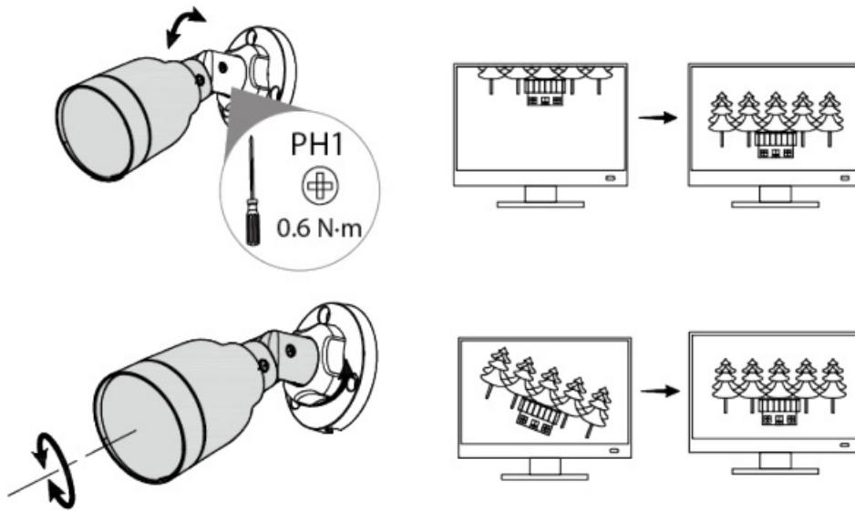
Figure 4-8 Adjust the lens angle
