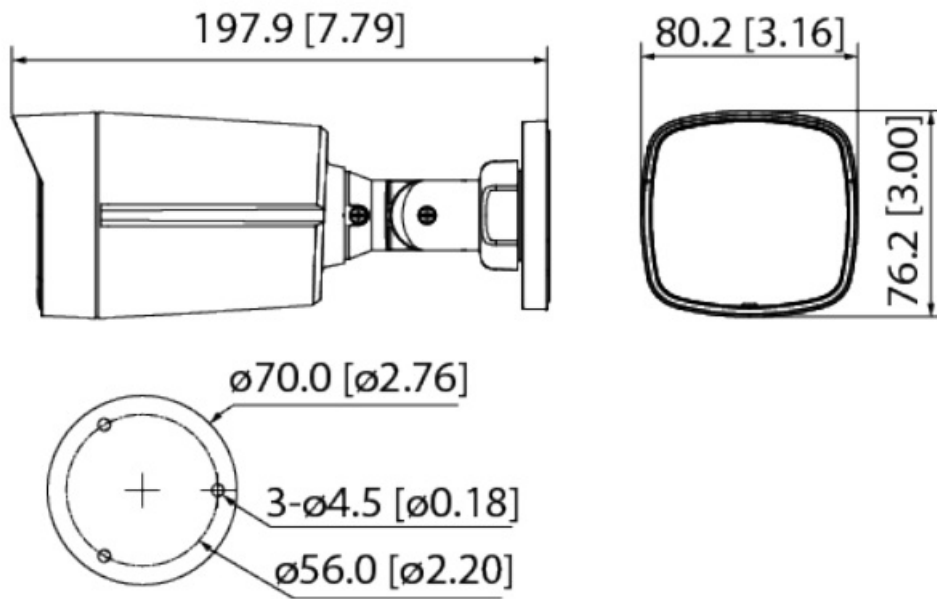
Figure 4-3 Dimensions: Model B (mm [inch])
