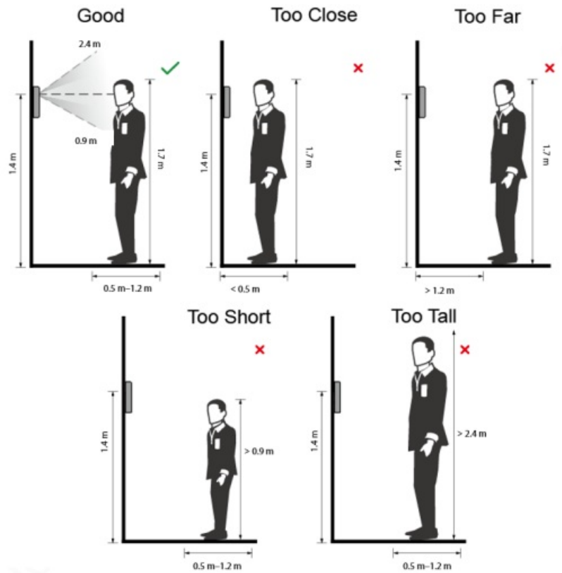
Appendix Figure 2-2 Appropriate face position
