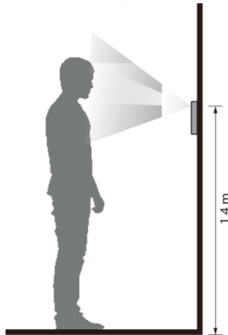
Figure 2-1 Installation height requirement
