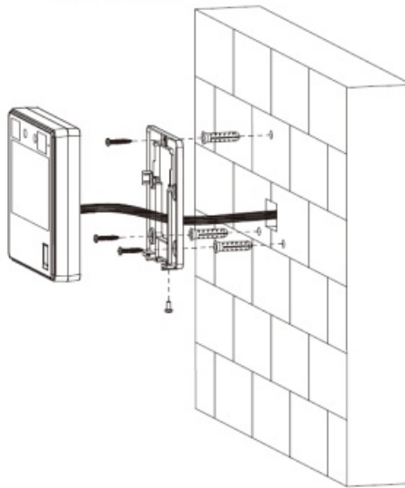
Figure 2-6 Wall mount
