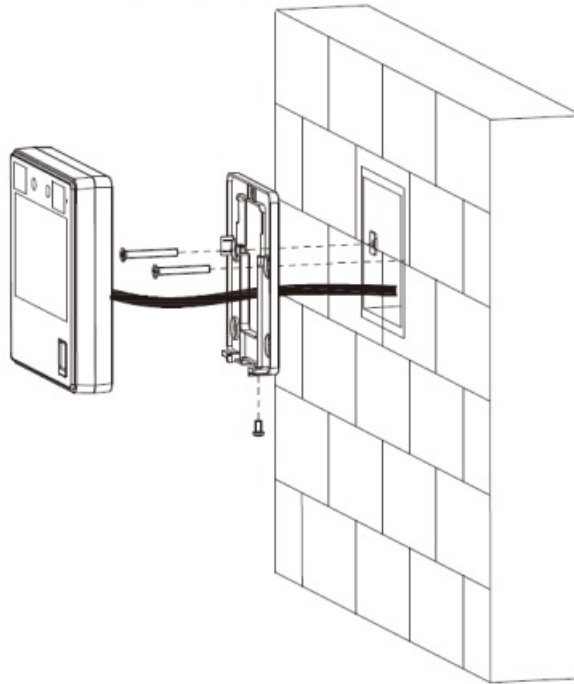
Figure 2 7 86 box mount
