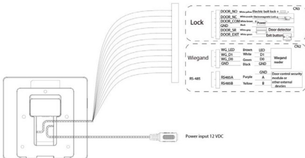
Figure 2-5 Wiring
