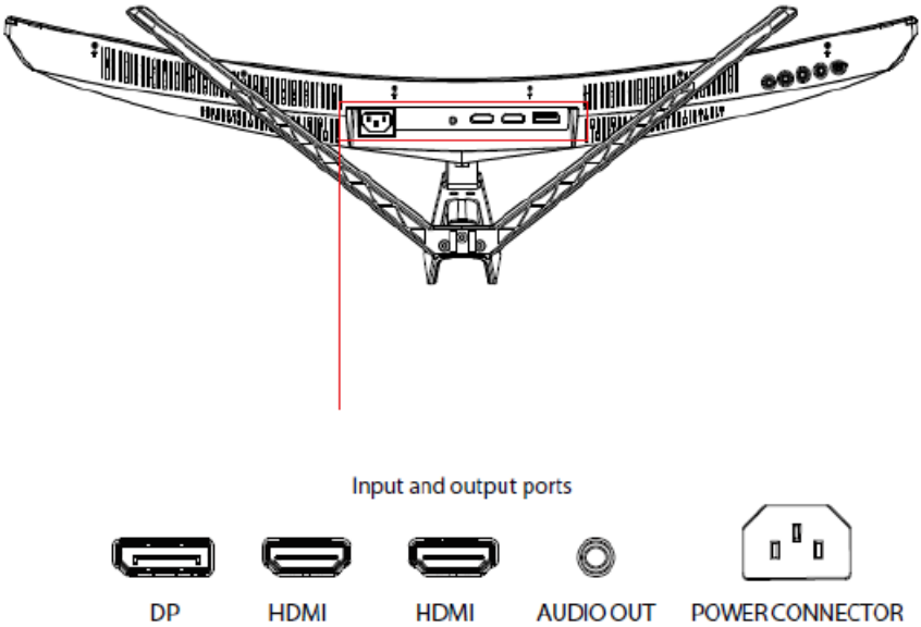
Figure 4-3 Input and output interface
