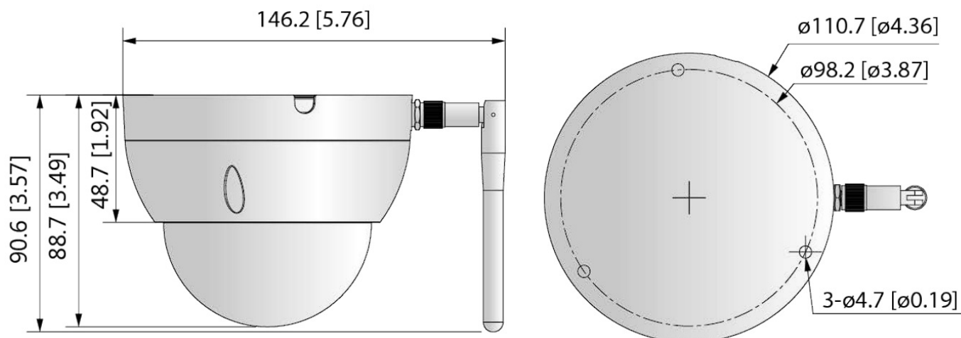
Figure 2-2 Dimensions (mm [inch])
