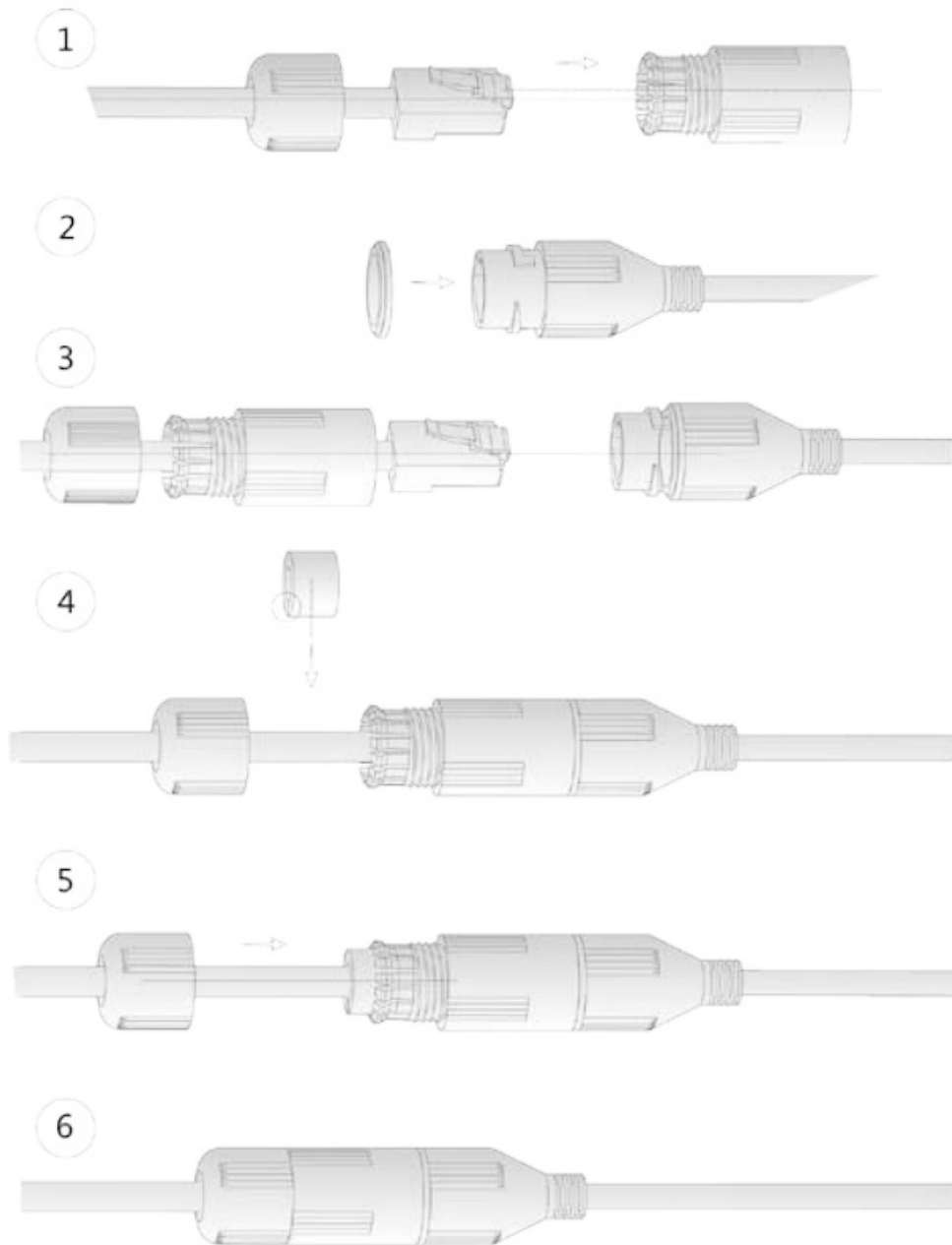
Figure 2-7 Install waterproof connector
