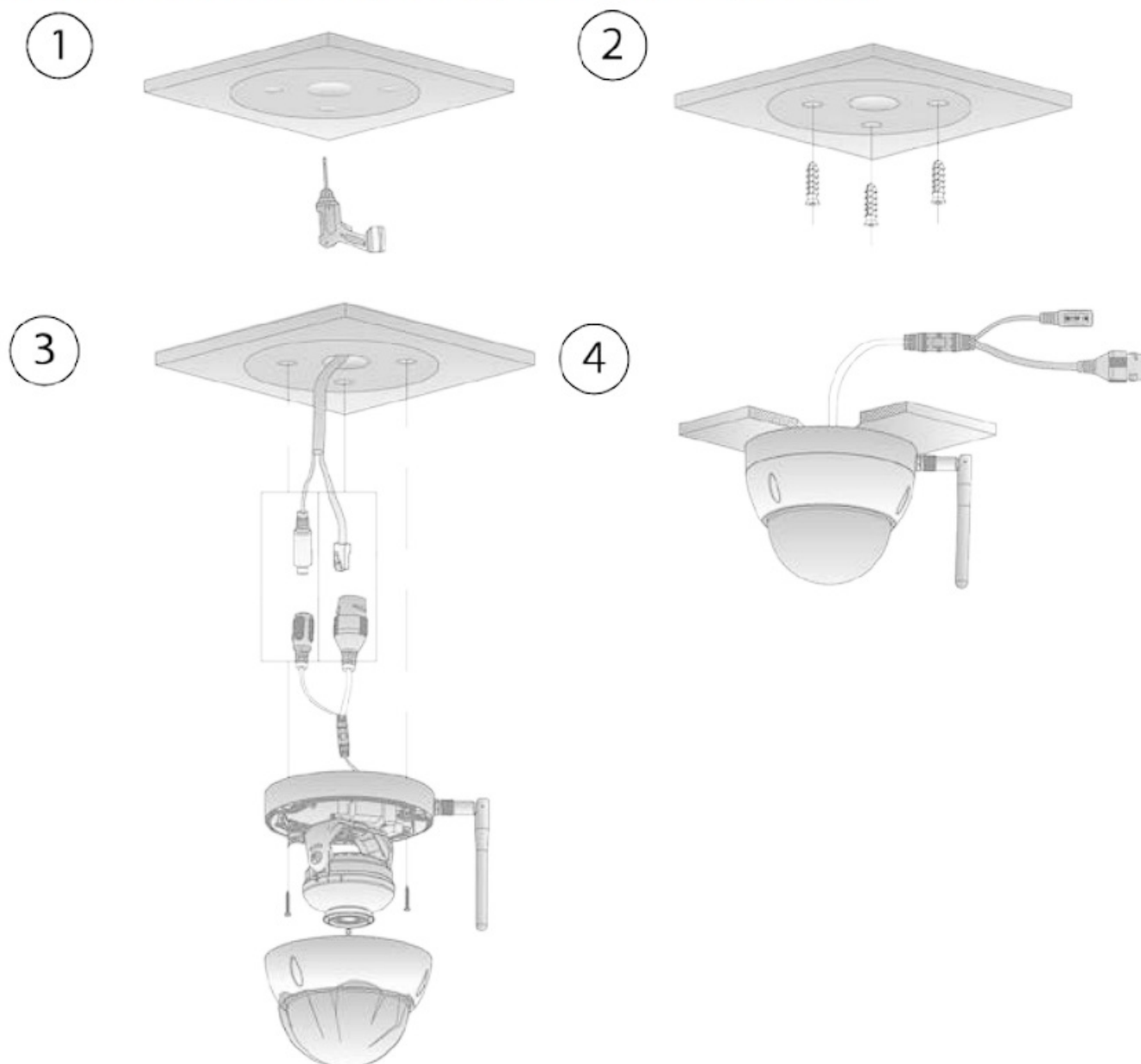
Figure 2-6 Cable going through the mounting surface
