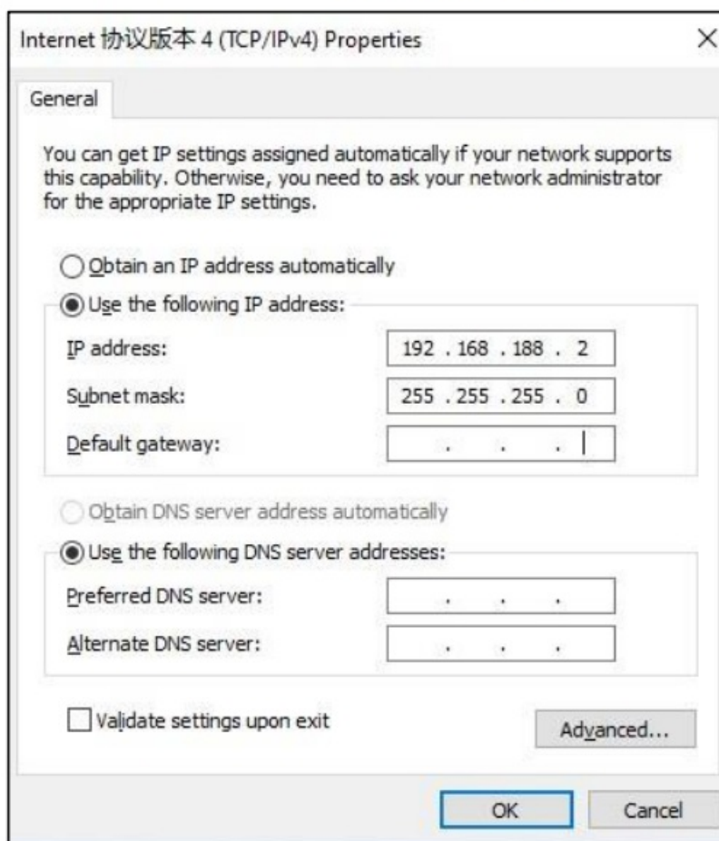
Figure 4-2 Set IP address
