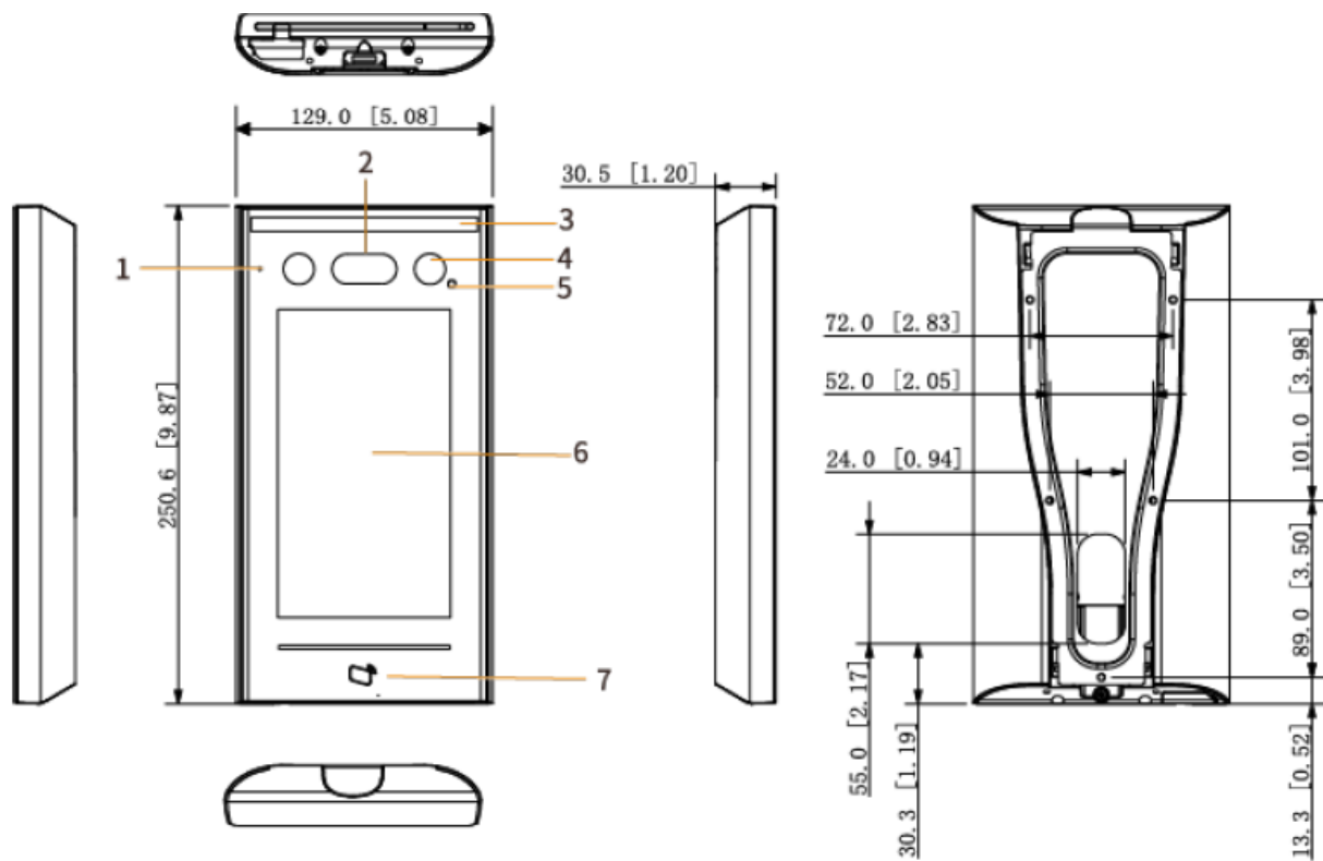
7-inch model X with fingerprint (unit: mm[inch])
