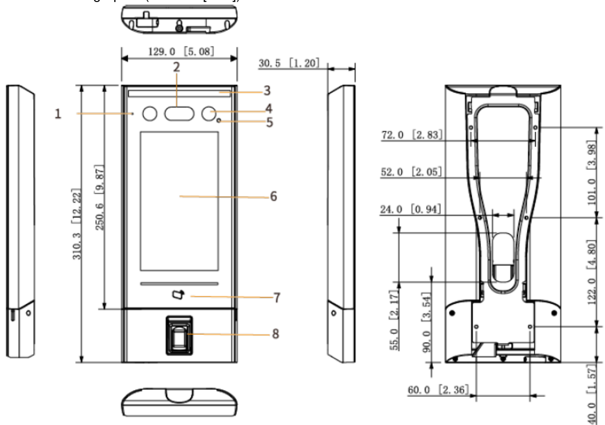
7-inch model X with fingerprint (unit: mm[inch])
