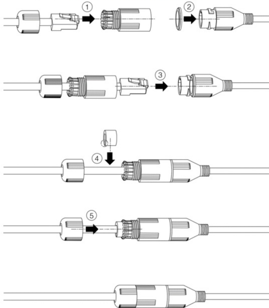
Figure 3-5 Install the waterproof connector
