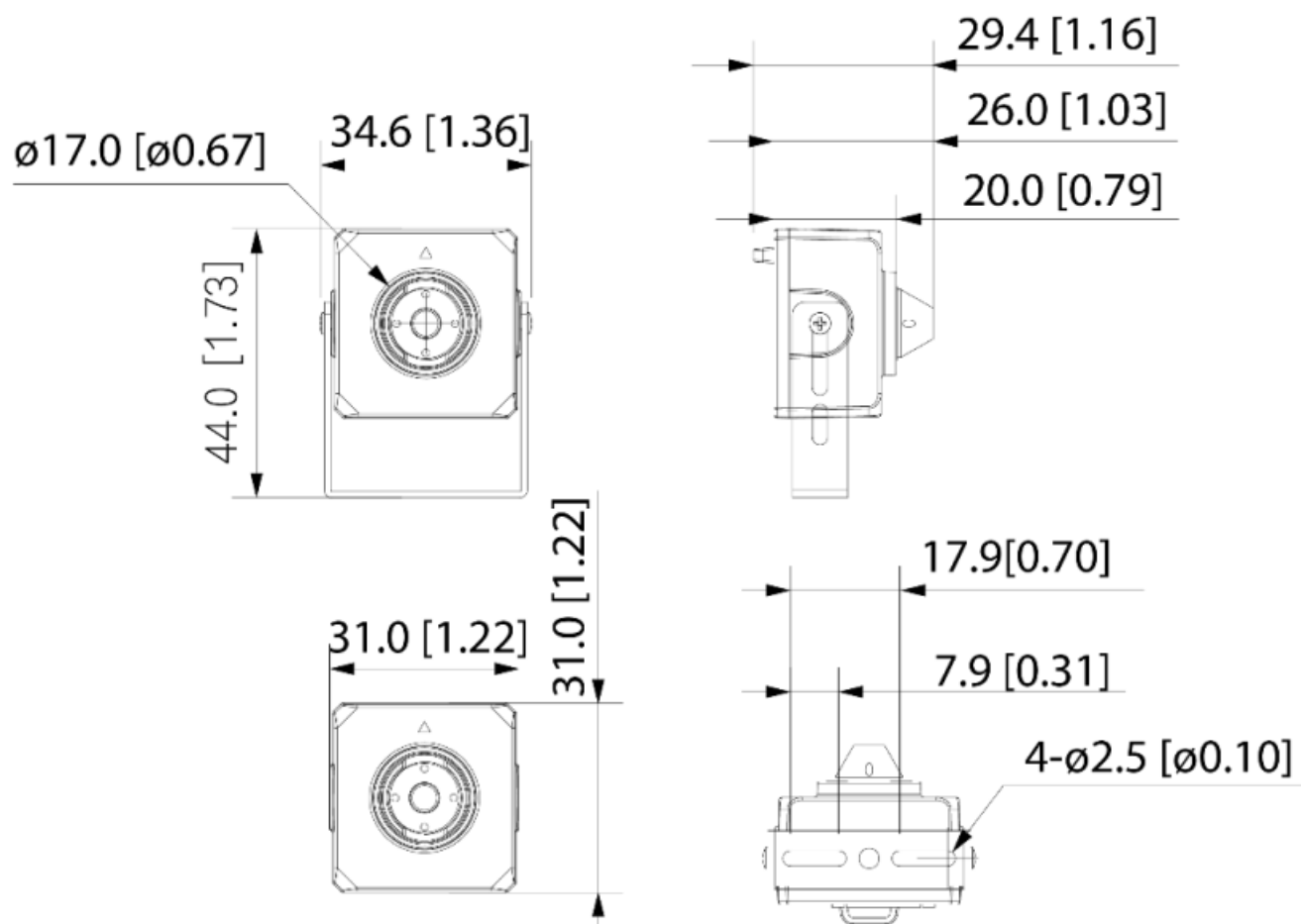
Figure 3-2 Dimensions (mm [inch])
