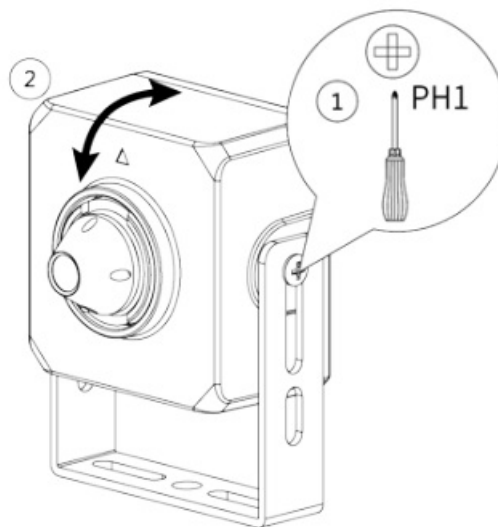
Figure 3-6 Adjust the lens angle
