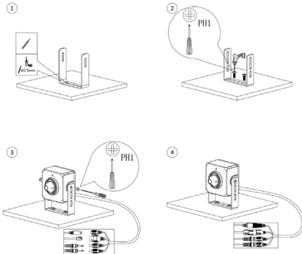
Figure 3-4 Attach the camera
