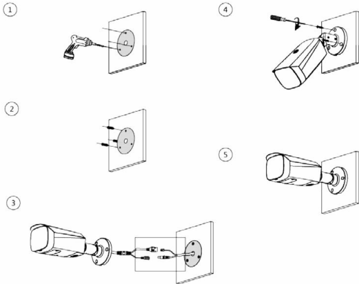
Figure 3-6 Cable going through the mounting surface
