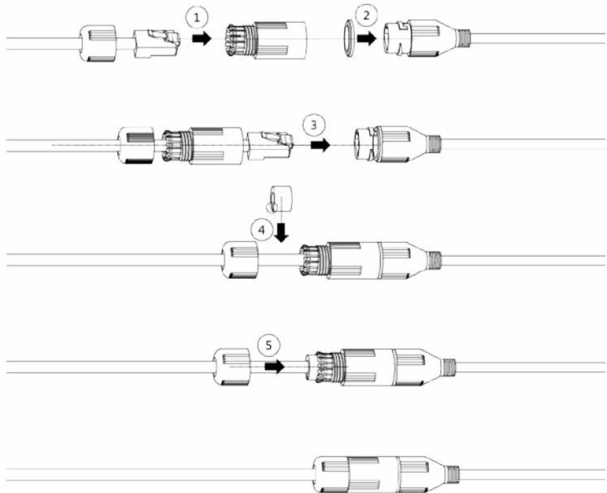
Figure 3-7 Install waterproof connector
