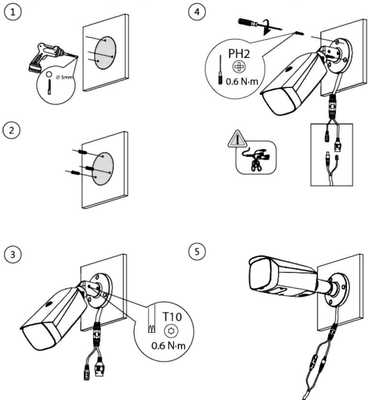
Figure 3-5 Cable going through the side cable tray
