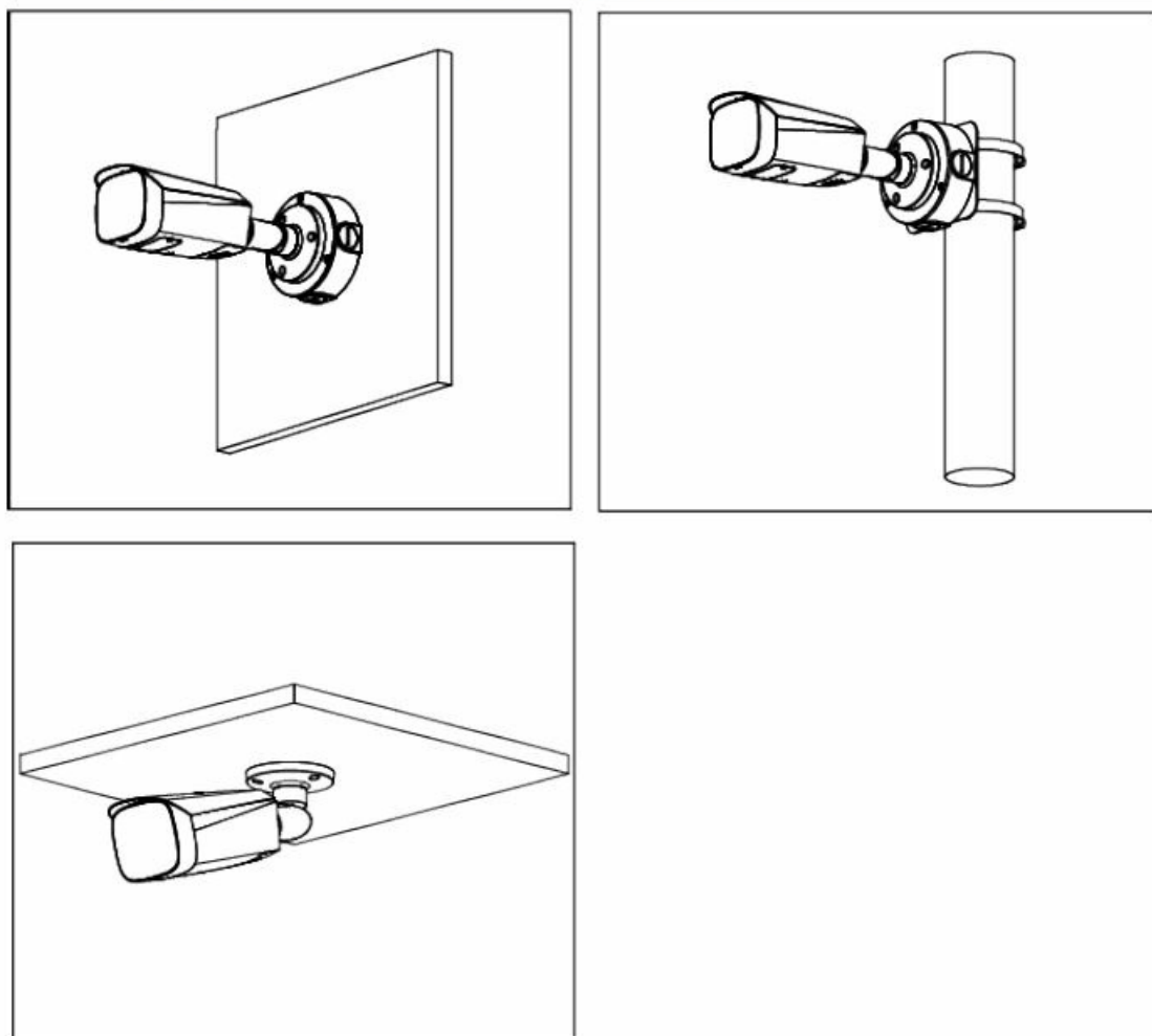
Figure 3-3 Installation methods
