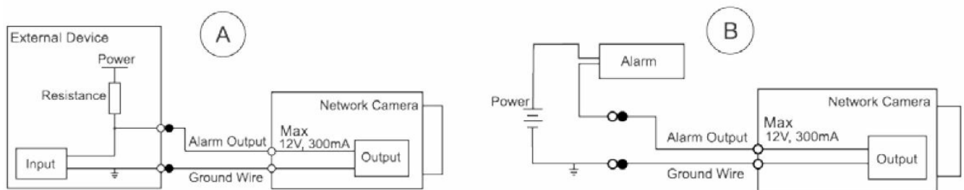
Figure 1-3 Alarm output
