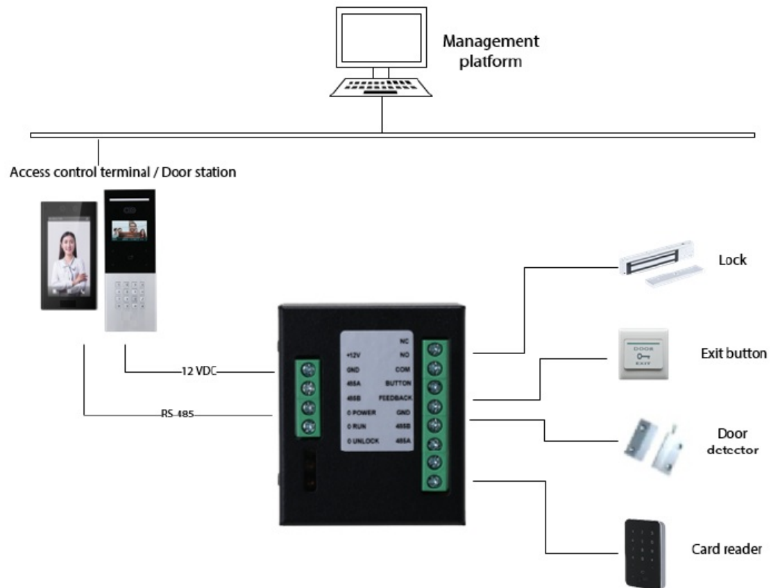
Figure 1-1 Networking diagram
