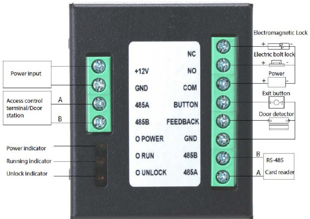
Figure 2-1 Ports
