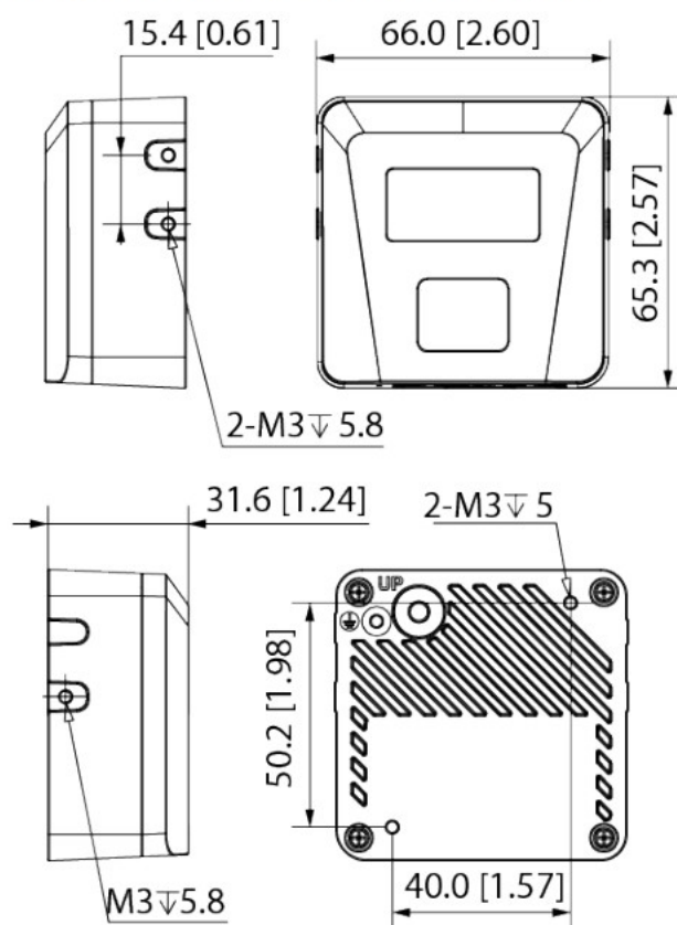
Figure 3-2 Dimensions (Unit: mm [inch])
