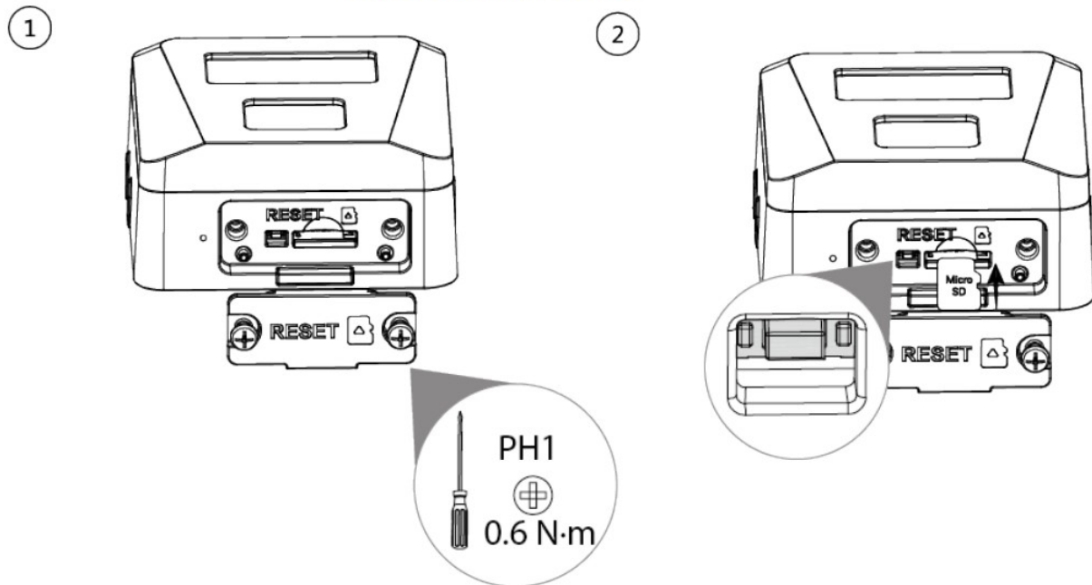
Figure 3-4 Install SD card
