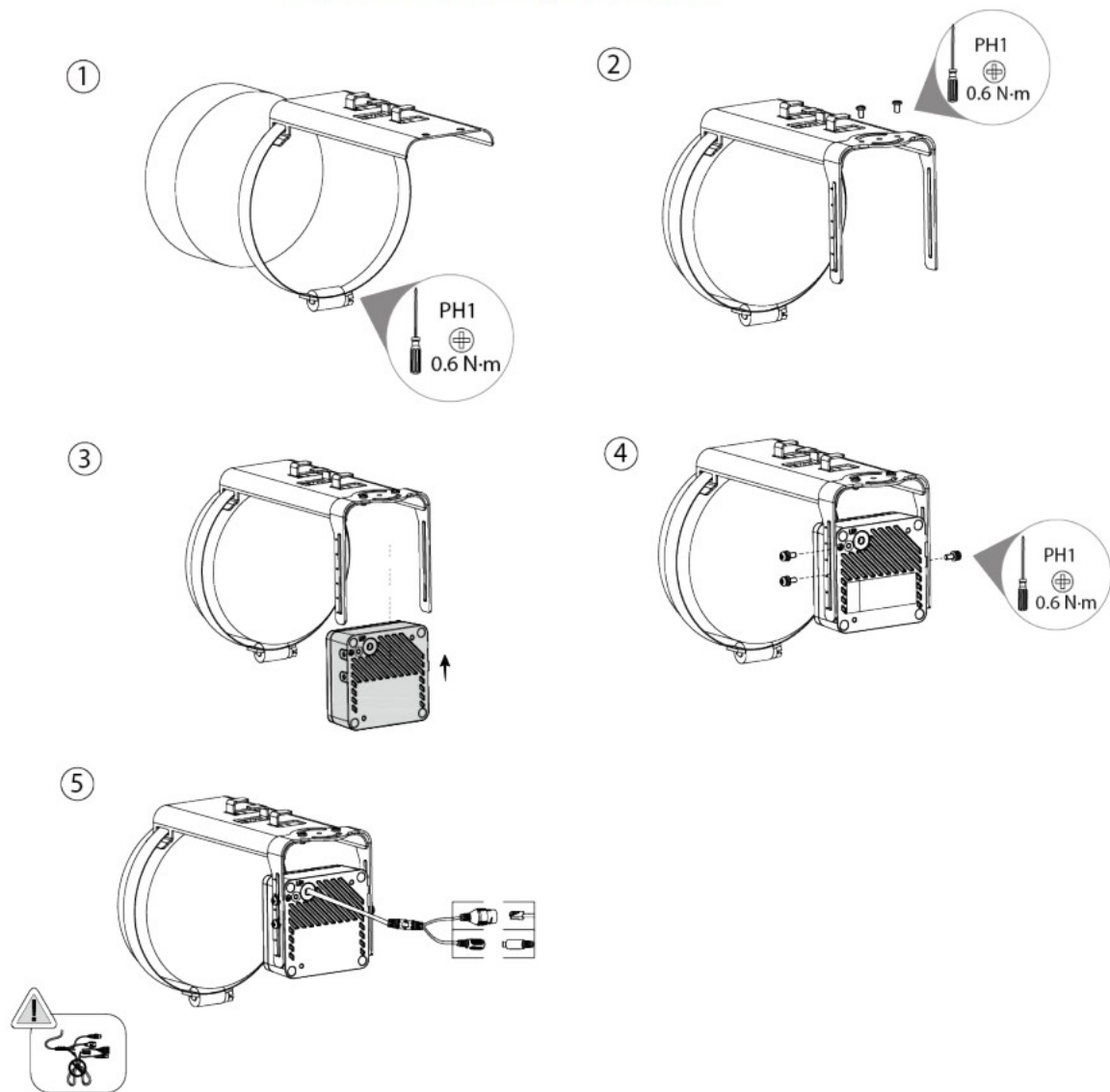
Figure 3-5 Attaching the Camera
