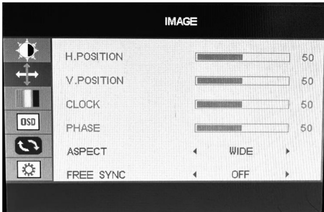
Figure 3-4 IMAGE
