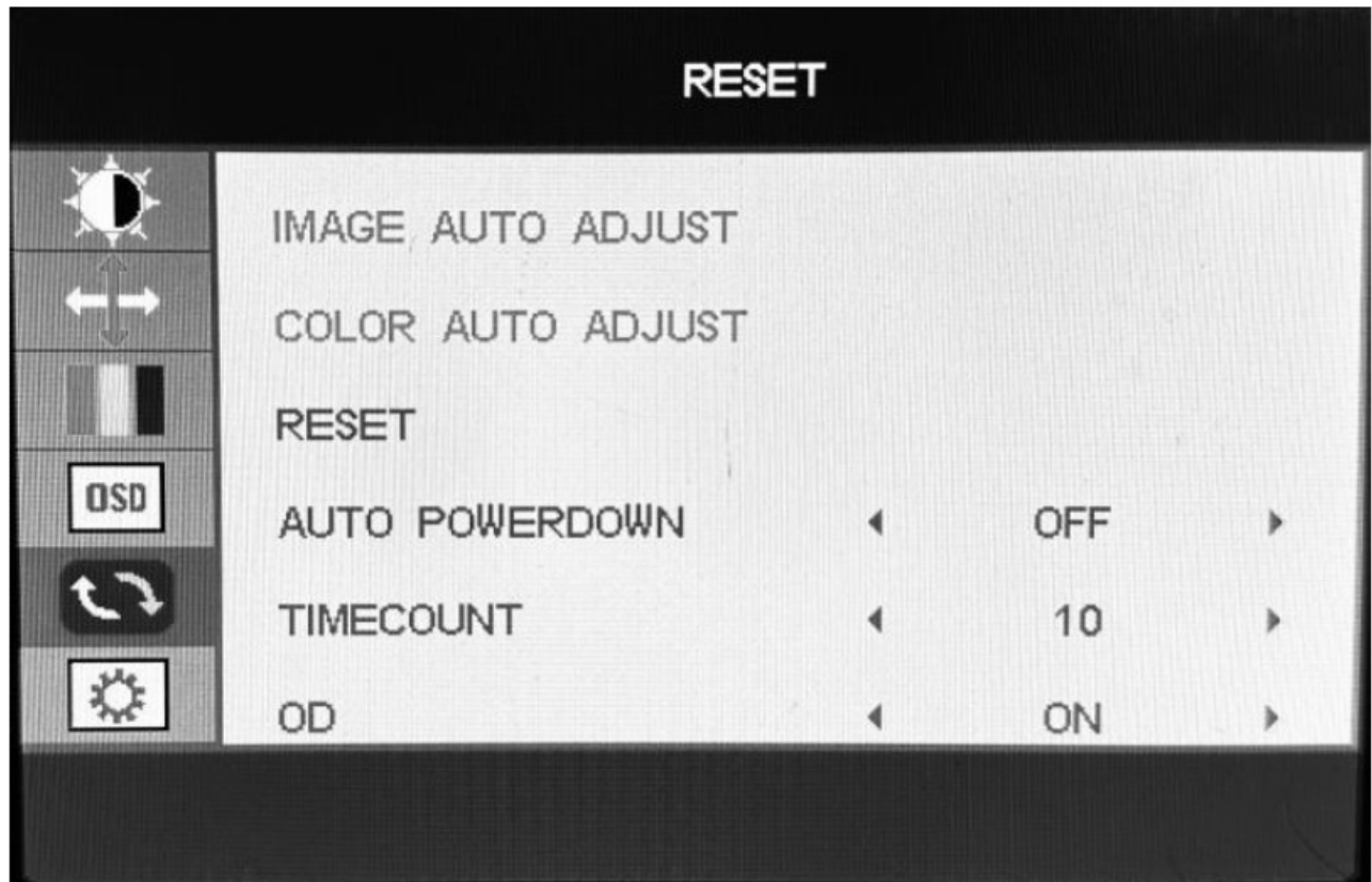
Figure 3-7 RESET
