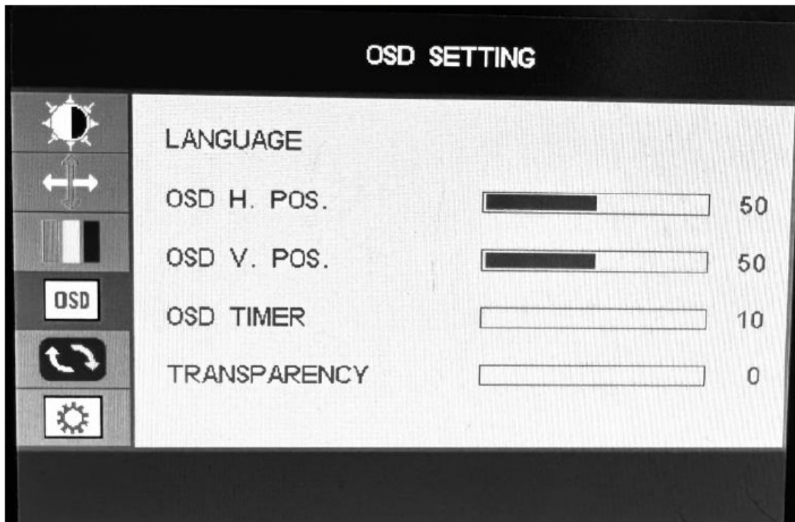
Figure 3-6 OSD SETTING
