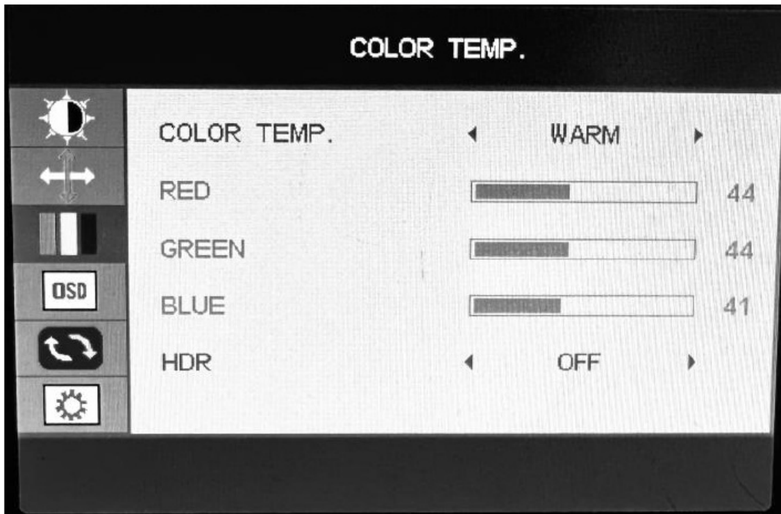
Figure 3-5 COLOR TEMP
