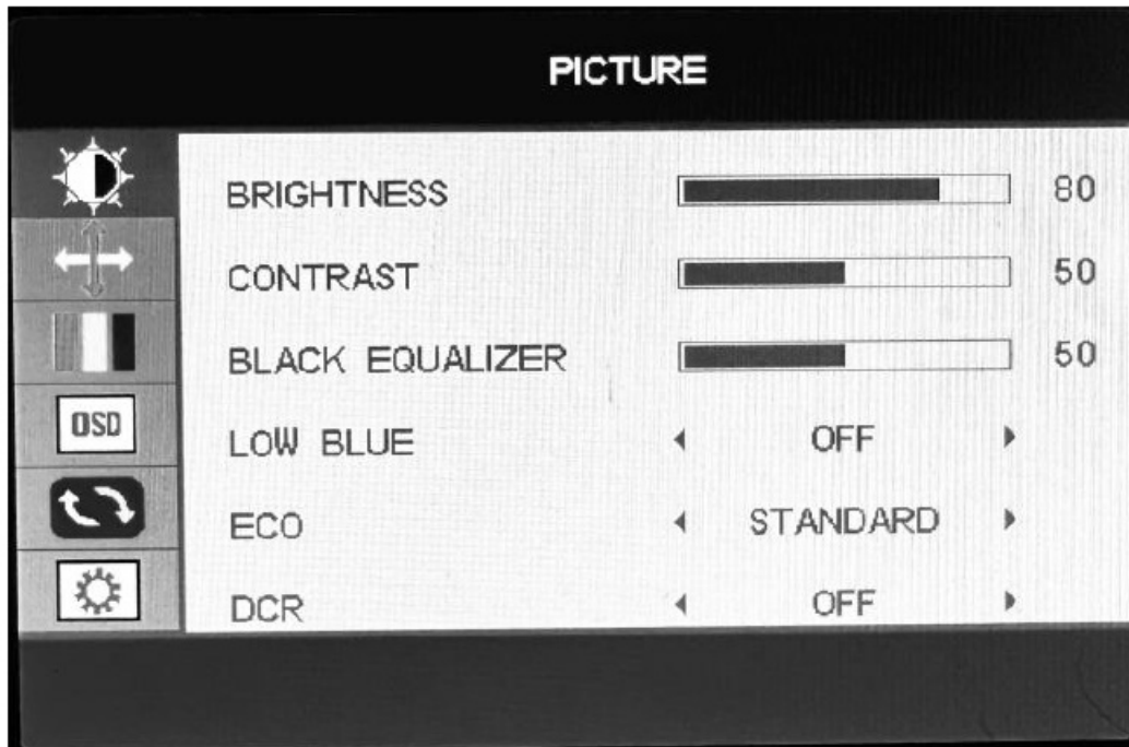
Figure 3-3 PICTURE
