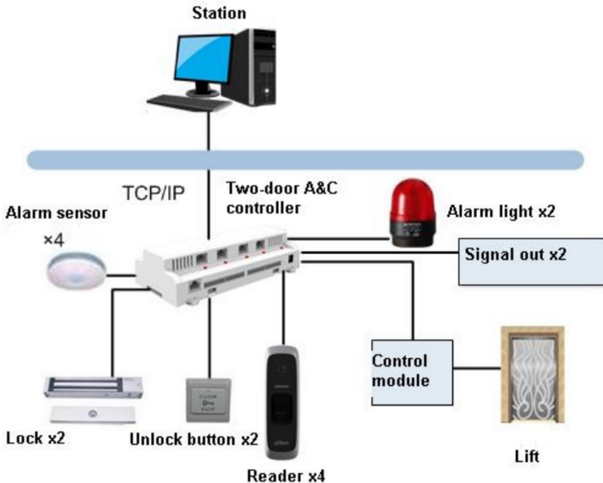
Figure 4-1 Installation
