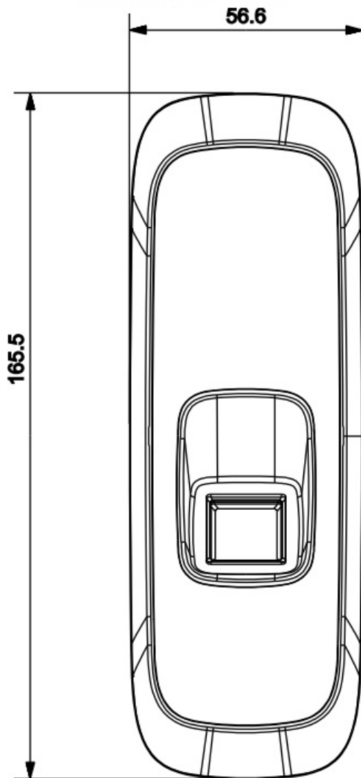
Figure 2-1 Front view
