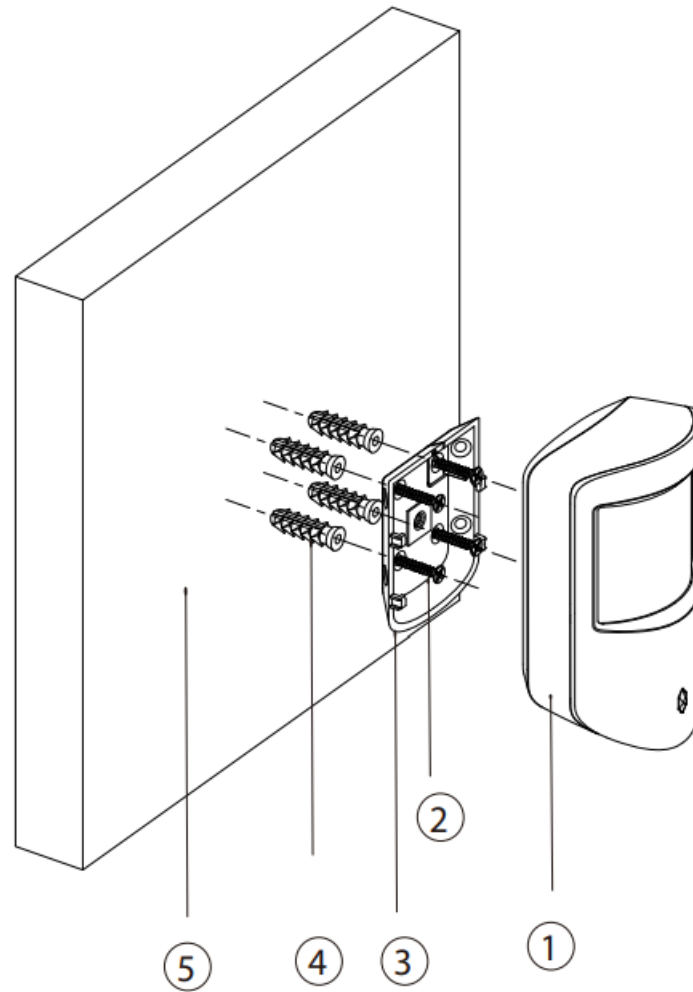
Figure 5-1 Installation items
