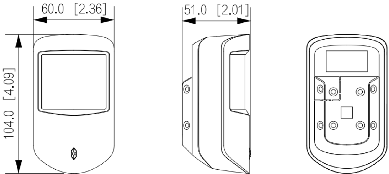
Figure 3-2 Dimensions (mm[inch])
