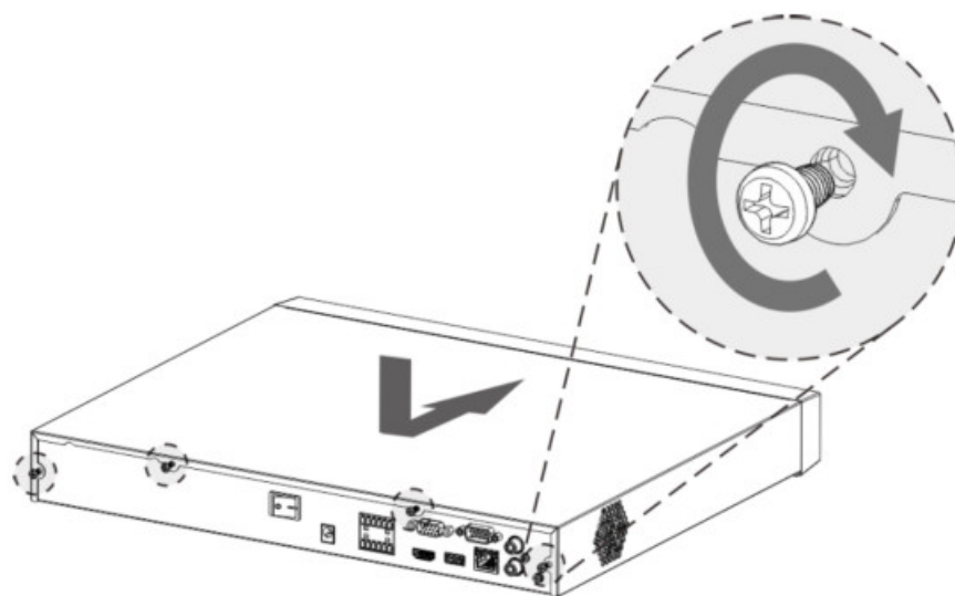
Figure 2-12 Installing HDD (6)
