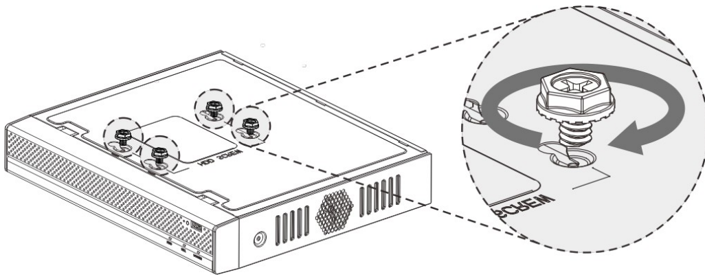
Figure 2-4 Installing HDD (4)
