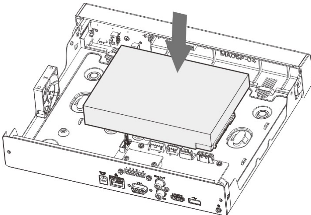
Figure 2-3 Installing HDD (3)
