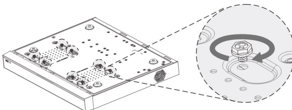
Figure 2-10 Installing HDD (4)
