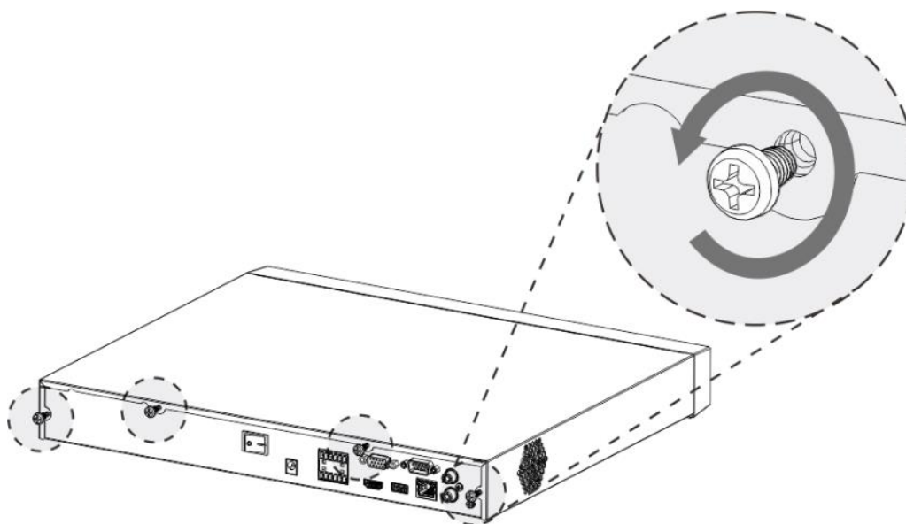
Figure 2-7 Installing HDD (1)
