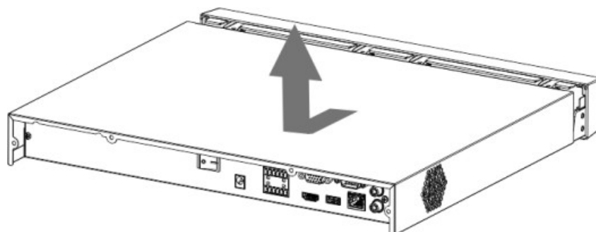
Figure 2-8 Installing HDD (2)
