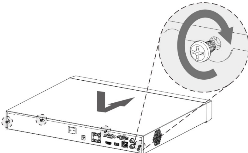
Figure 2-6 Installing HDD (6)
