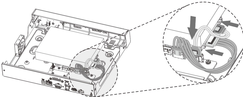
Figure 2-5 Installing HDD (5)
