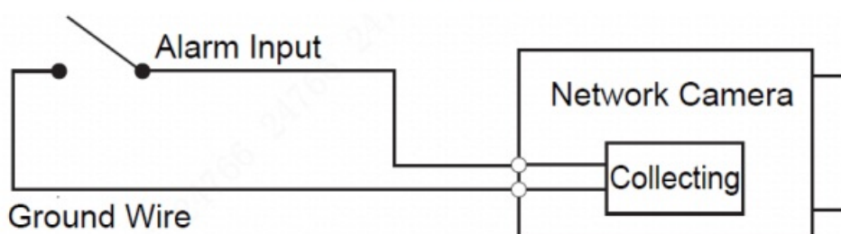
Figure 1-2 Alarm input
