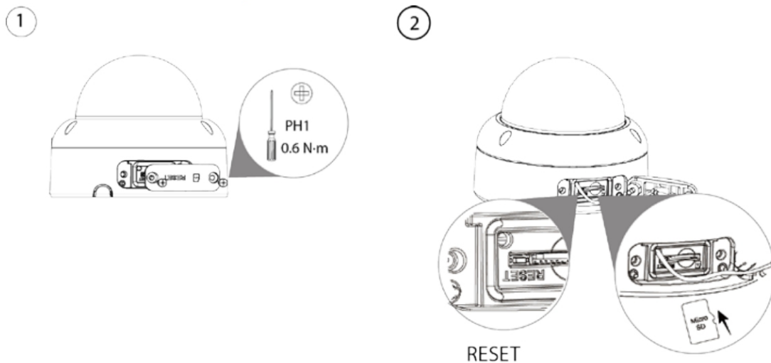
Figure 3-4 Install SD card
