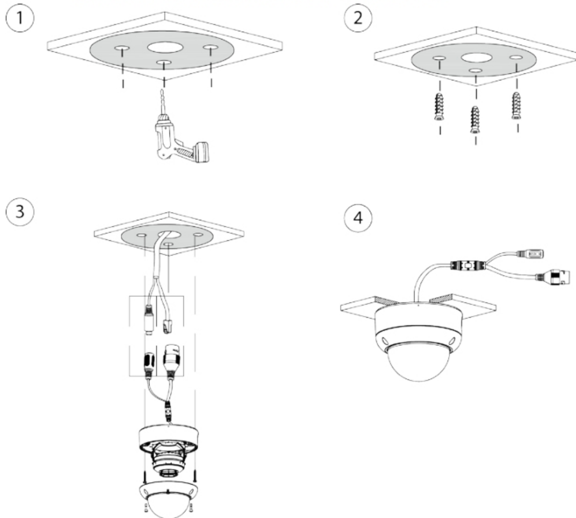
Figure 3-7 Cable going through the mounting surface
