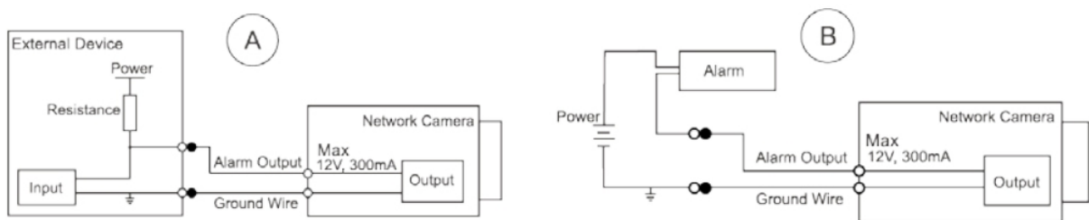
Figure 1-3 Alarm output
