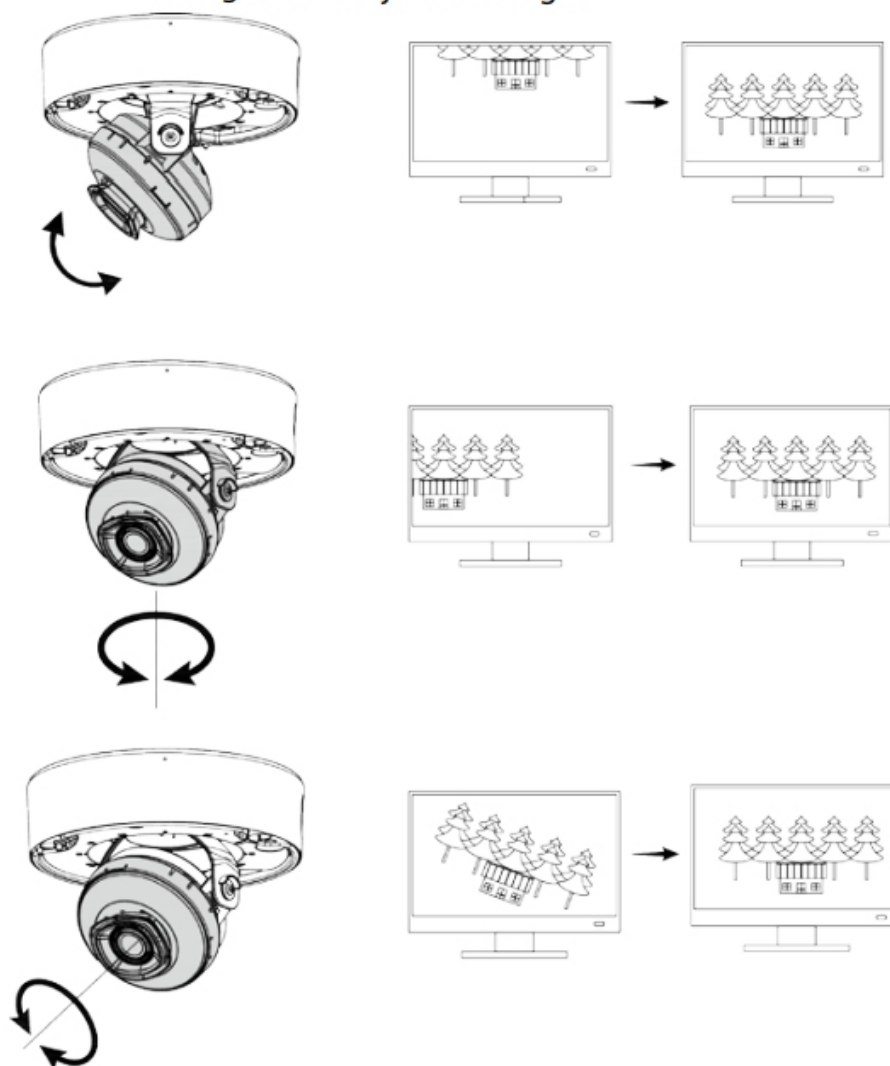
Figure 3-9 Adjust lens angle
