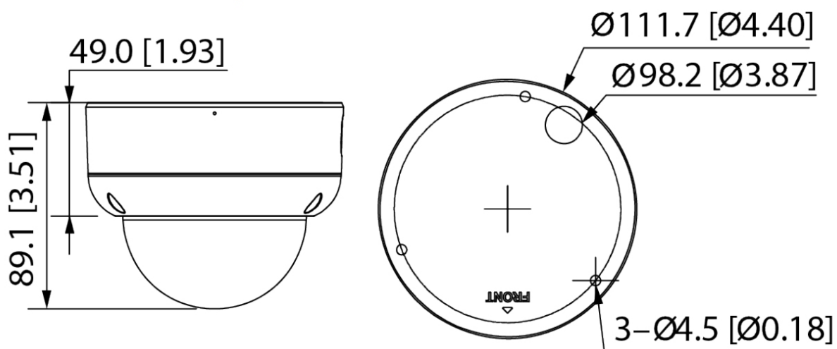
Figure 3-2 Dimensions (mm [inch])
