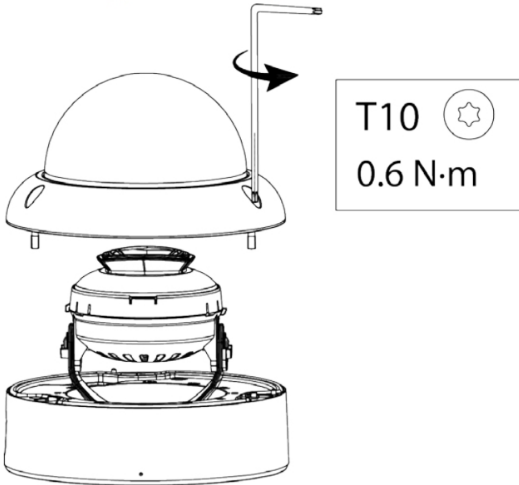
Figure 3-5 Detaching camera
