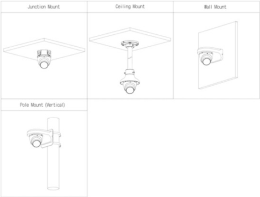
DH-PFB204W-G Wall mount bracket
